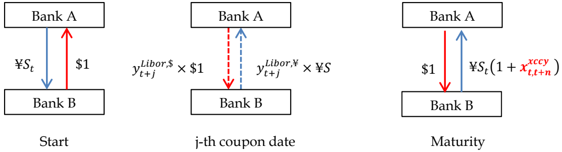
Figure 3: Cash Flow Diagram for JPY/USD Cross-Currency Basis Swap: This figure shows the cash flow exchanges of a standard yen/dollar cross-currency basis swap. At the inception of the swap, Bank A receives $1 from Bank B in exchange of ¥S_t . At the j -th coupon date, Bank A pays a dollar floating cash flow equal to y_{t+j}^{Libor,\$} percent on the $1 notional to Bank B, where y_{t+j}^{Libor,\$} is the three-month U.S. dollar Libor at time t + j . In return, Bank A receives from Bank B a floating yen cash flow equal to (y_{t+j}^{Libor,¥} + x_{t,t+n}^{xccy}) on the ¥S_t notional, where y_{t+j}^{Libor,¥} is the three-month yen Libor at time t + j , and x_{t,t+n}^{xccy} is the cross-currency basis swap spread, which is pre-determined at date t at the inception of the swap transaction. When the swap contract matures, Bank B receives $1 from Bank A in exchange of ¥S_t , undoing the initial transaction.
