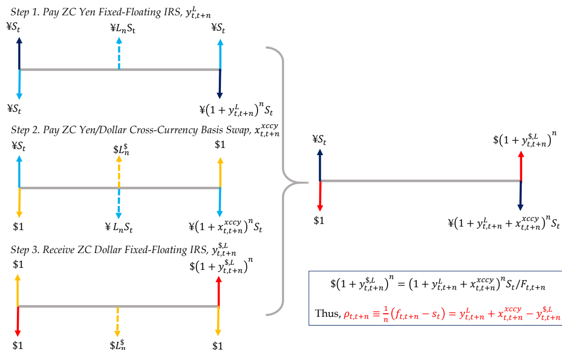
Figure 4: Cash Flow Diagram for Long-Term Forward Premium: This figure shows that the long-term forward premium is equal to the zero fixed-for-fixed cross-currency swap rate. The zero-coupon fixed-for-fixed cross-currency swap can be constructed using the following three steps: (1) paying a zero-coupon foreign currency fixed for floating interest rate swap indexed to the foreign currency Libor; (2) paying a zero-coupon foreign currency-Libor for USD-Libor cross-currency basis swap; and (3) receiving a USD fixed for floating interest rate swap. By summing up cash flows of the three steps, all floating cash flows are canceled and we are left exchanges of fixed cash flows at the inception and maturity of the swap in two currencies.
