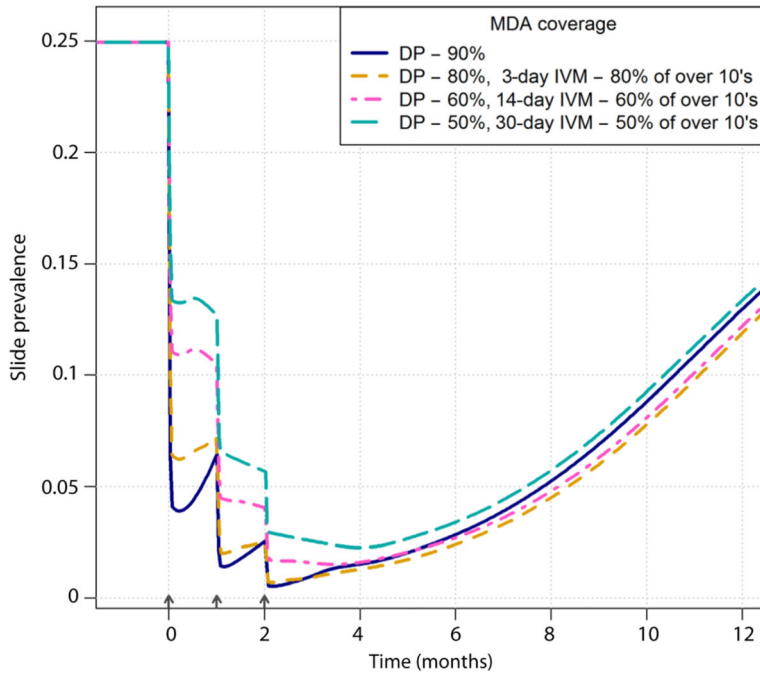
Fig. 5. Mathematical malaria transmission model
