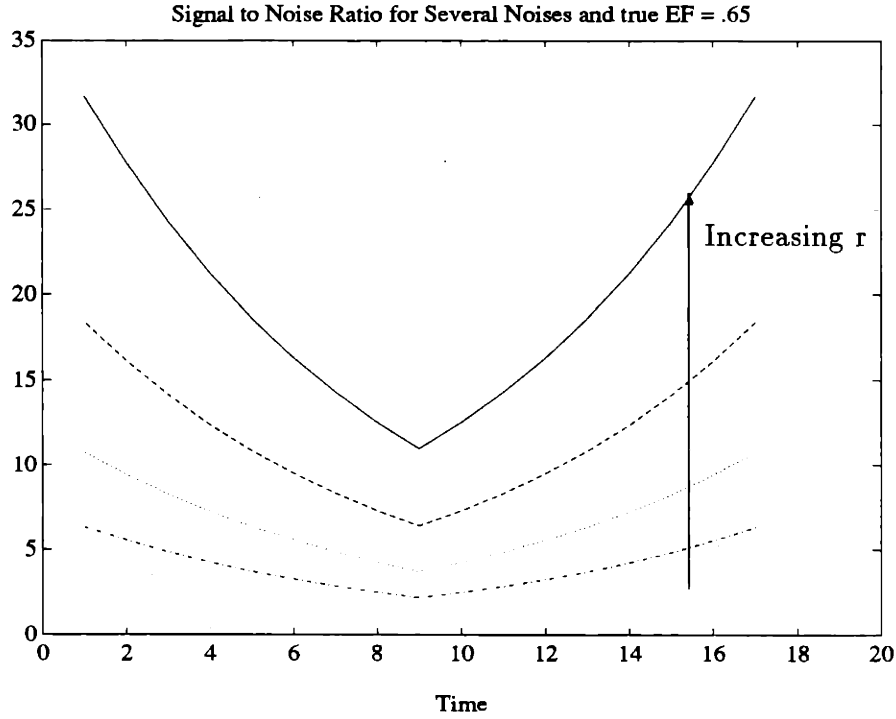
Figure 5-3: Signal to Noise Ratios for several noises with true EF = .65
