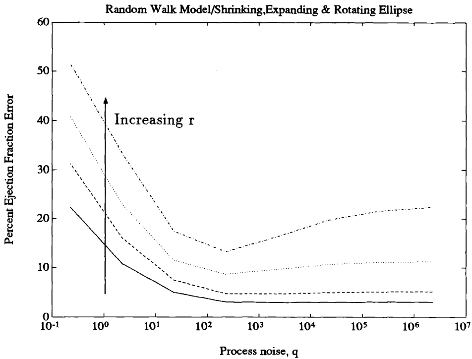
Figure 4-20: Ejection Fraction error using random walk model for dynamics. Each curve corresponds to a different value of measurement noise, r
