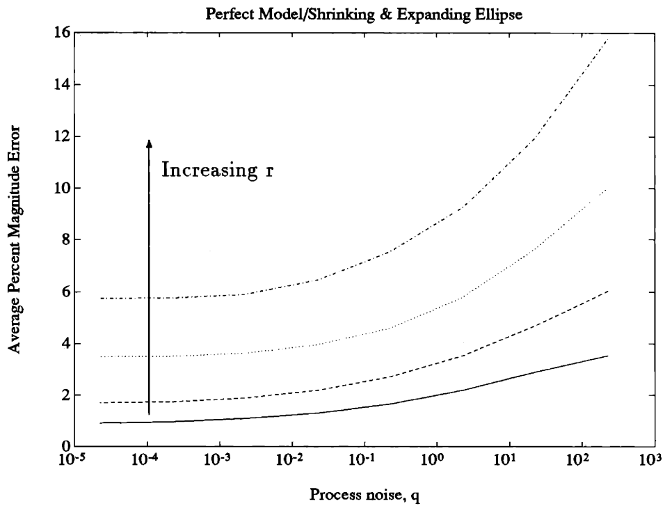
Figure 4-8: Average of percent magnitude error over time and over 100 runs. Uses perfect model of dynamics. Each curve corresponds to a different value of measurement noise, r
