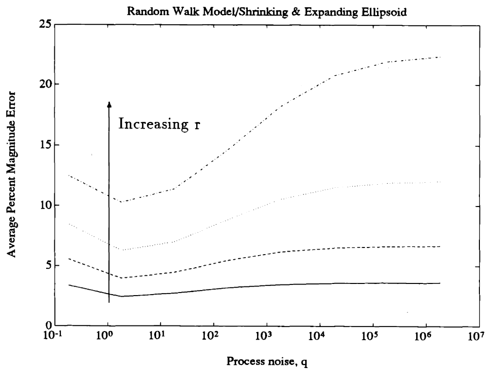
Figure 4-26: Average percent magnitude error using random walk model of dynamics. Each curve corresponds to a different value of measurement noise, r .
