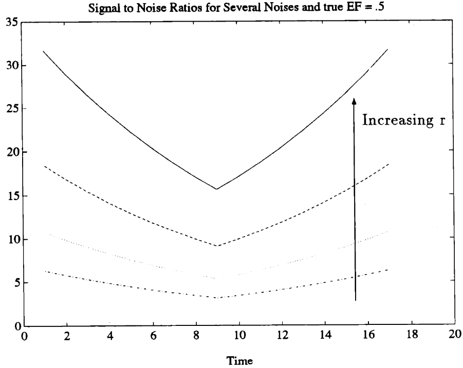
Figure 5-7: Signal to Noise Ratios for several noises with true EF = .5
