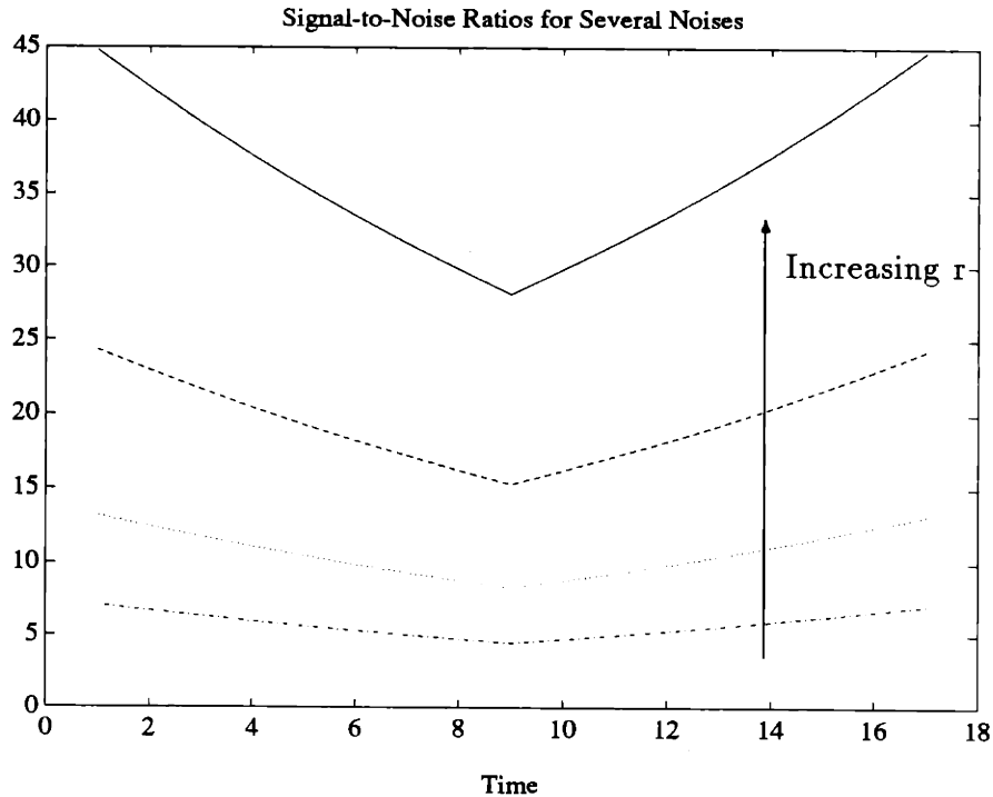
Figure 4-21: Several Signal-to-Noise Ratios for Three Dimensional Reconstruction
