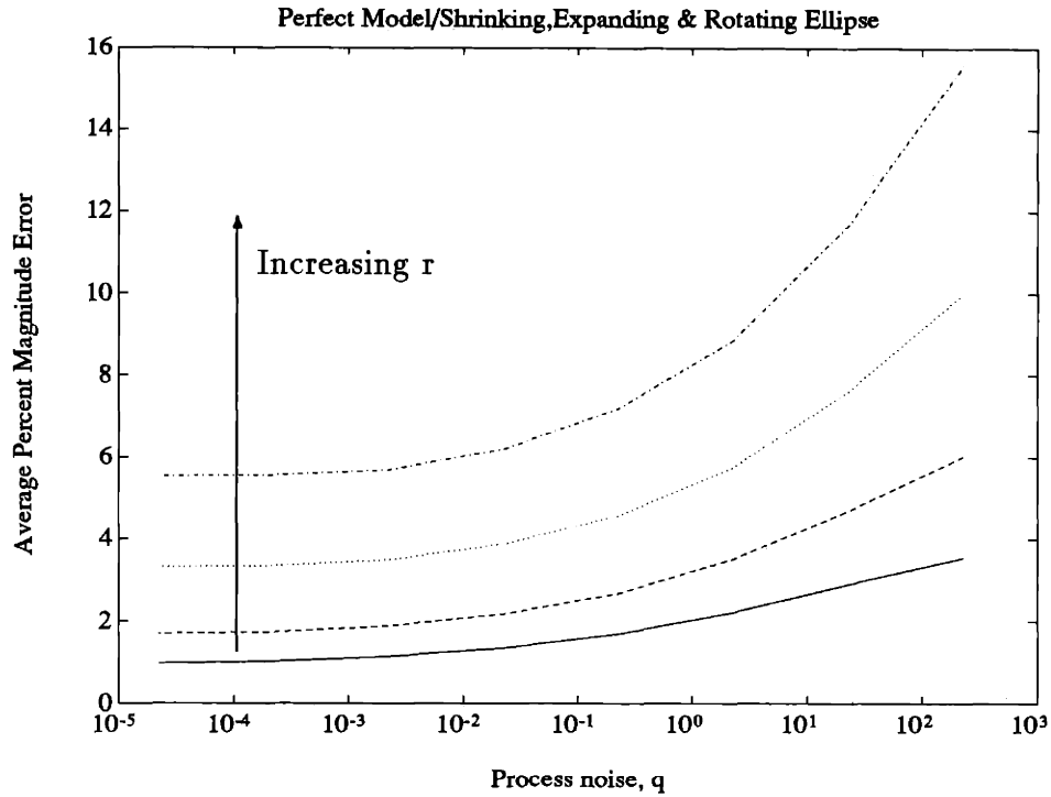
Figure 4-15: Average percent magnitude error using perfect model for dynamics. Each curve corresponds to a different value of measurement noise, r
