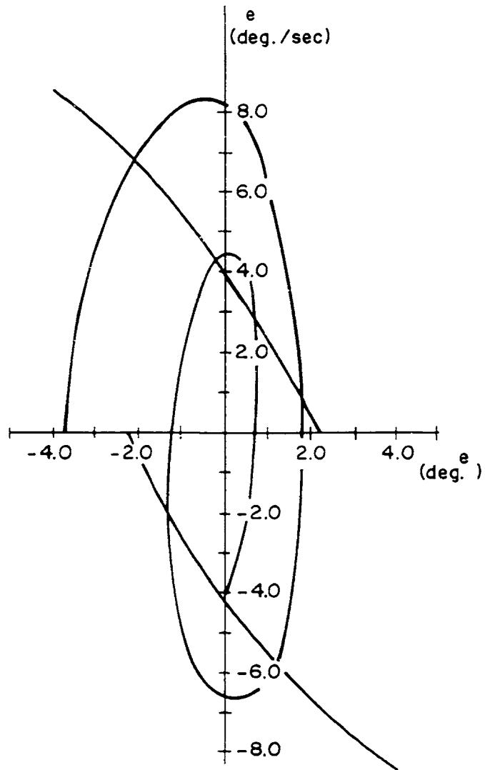
Fig. 7.5 Calculated Phase Portrait and Switching Lines
