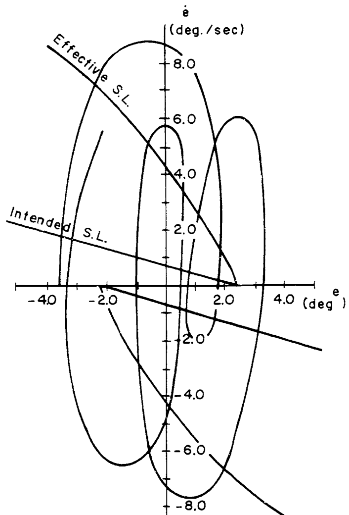
Fig. 7.4 Experimental Trajectory and Switching Lines
