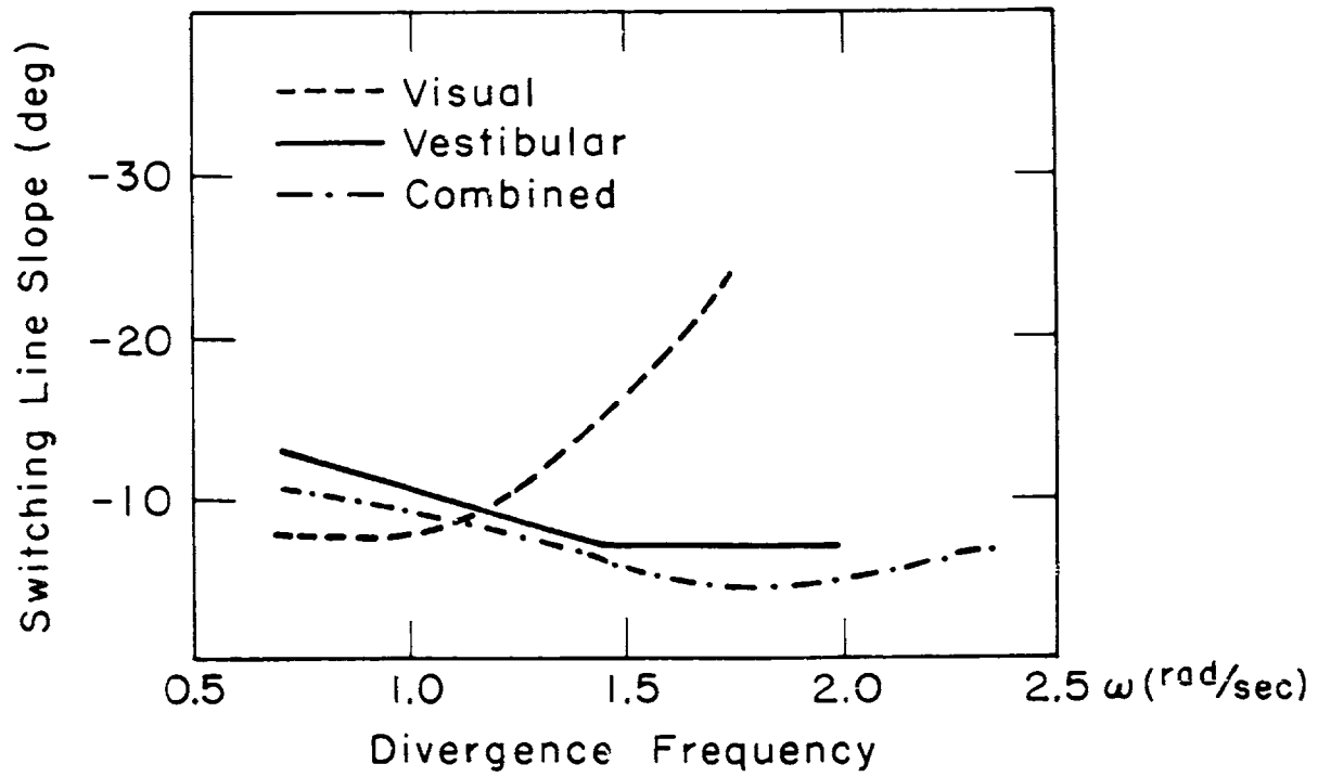
Fig. 7.6 Switching Line Slope for Control of Inverted Pendulum
