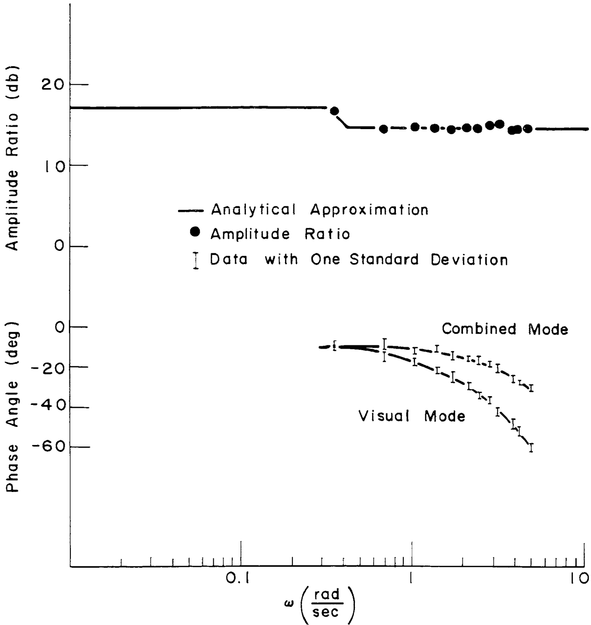
Fig. 6.3 Describing Function of The Human Operator in Visual and Combined Mode. Horizontal Rotation
