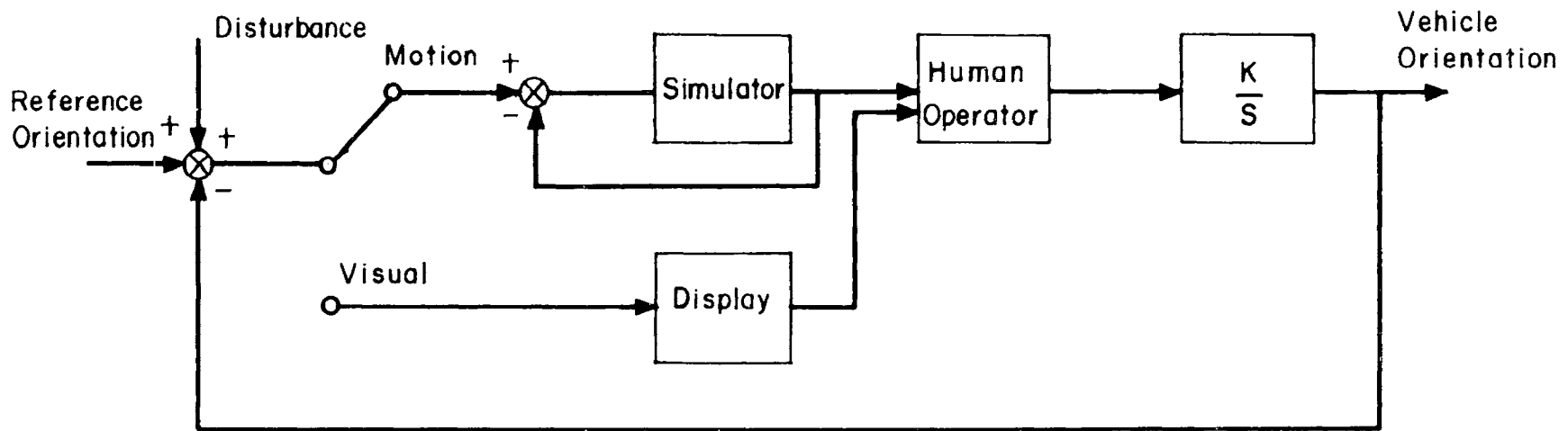
Fig. 6.2 Velocity Control with Visual or Motion Mode
