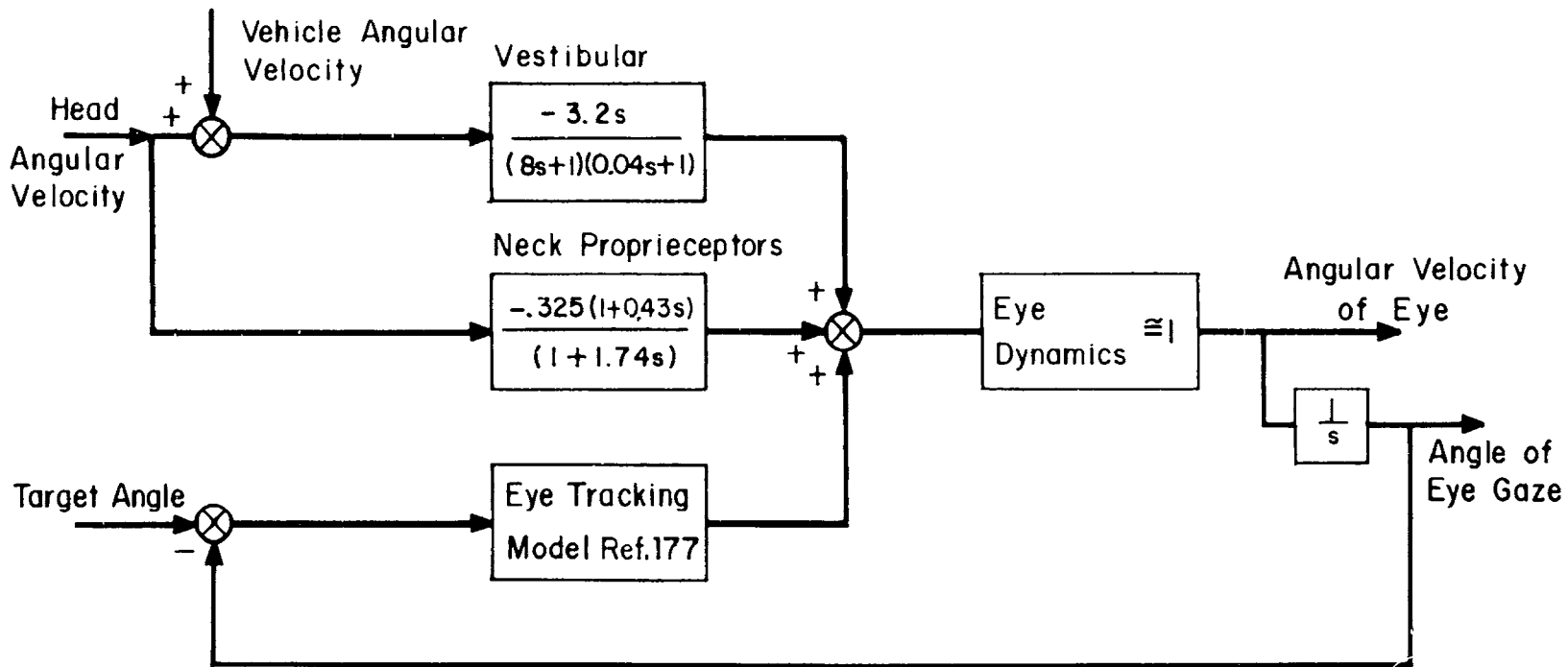
Fig. 5.14 Model for Multi-input Horizontal Eye Movement Control System
