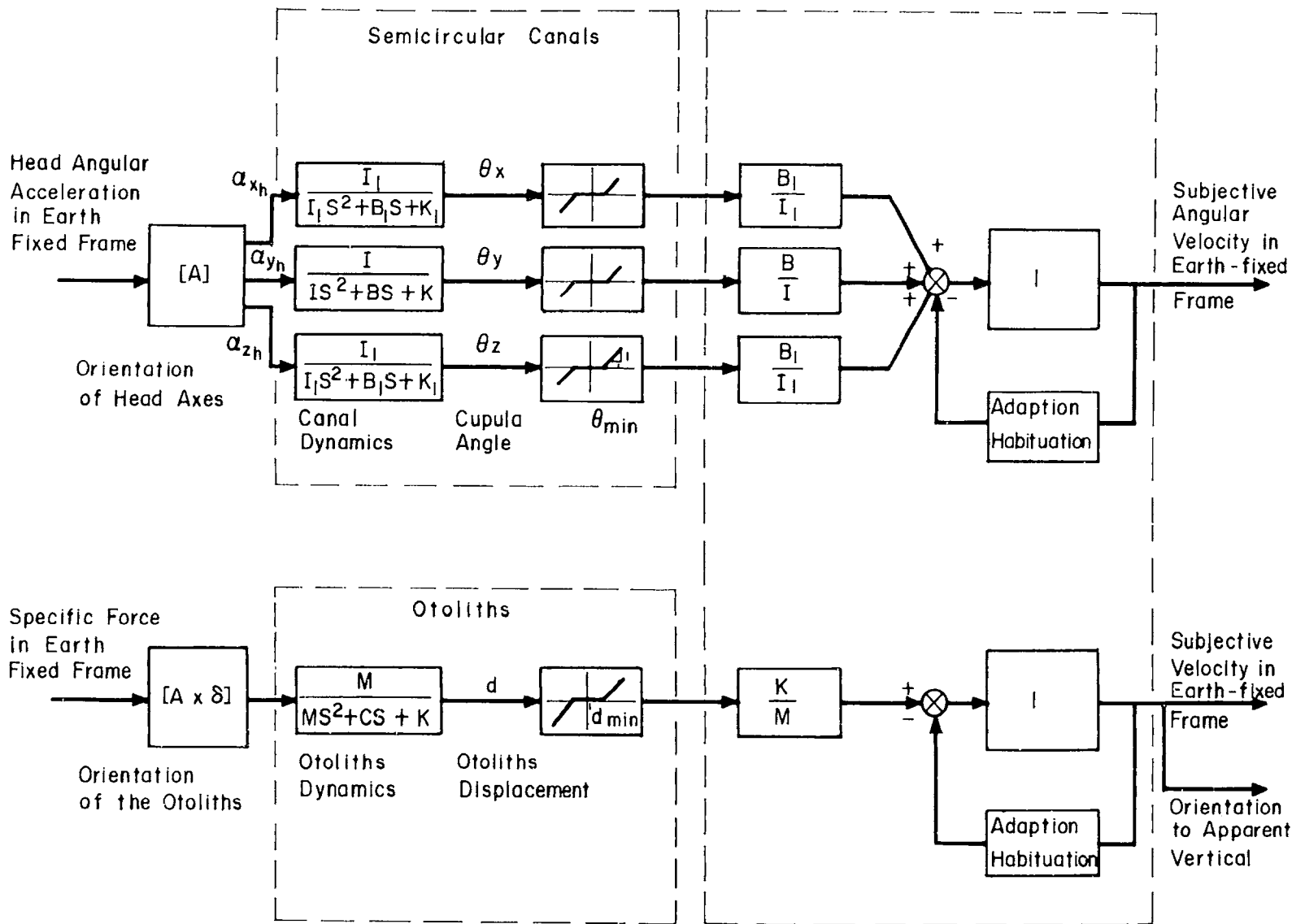
Fig. 8.1 Block Diagram of the Vestibular System
