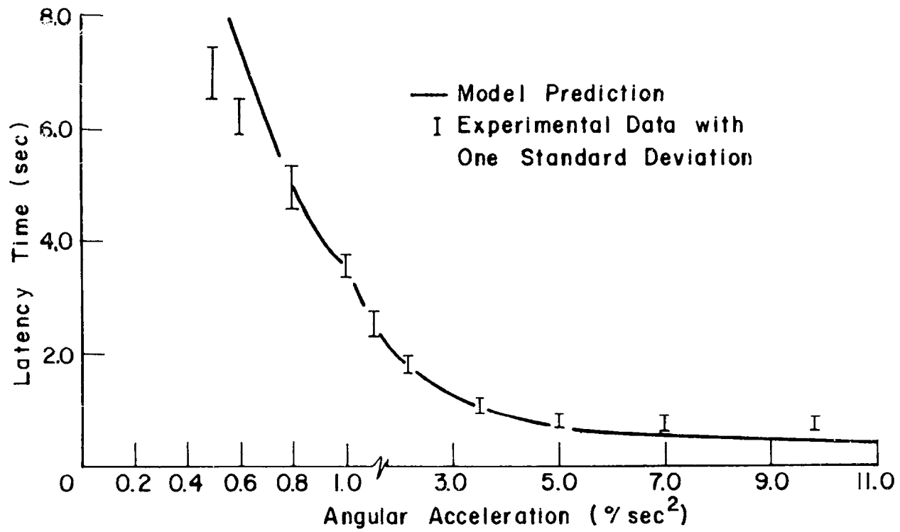
Fig. 3.6 Latency Times for Perception of Angular Accelerations about The Roll Axis ( X_h ) Note : Scale Change of Angular Acceleration
