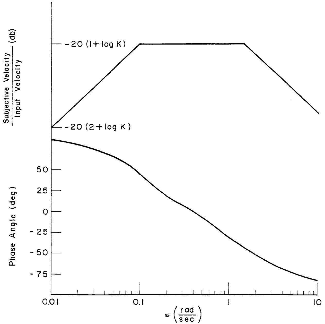
Fig. 4.4 Bode Plot of Otoliths Model
