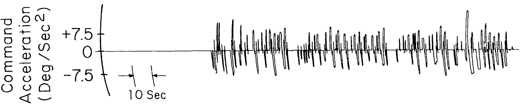
Fig. 7.2 Time-Record-Control of Inverted Pendulum Showing Bang-Bang Use of Linear Controller
