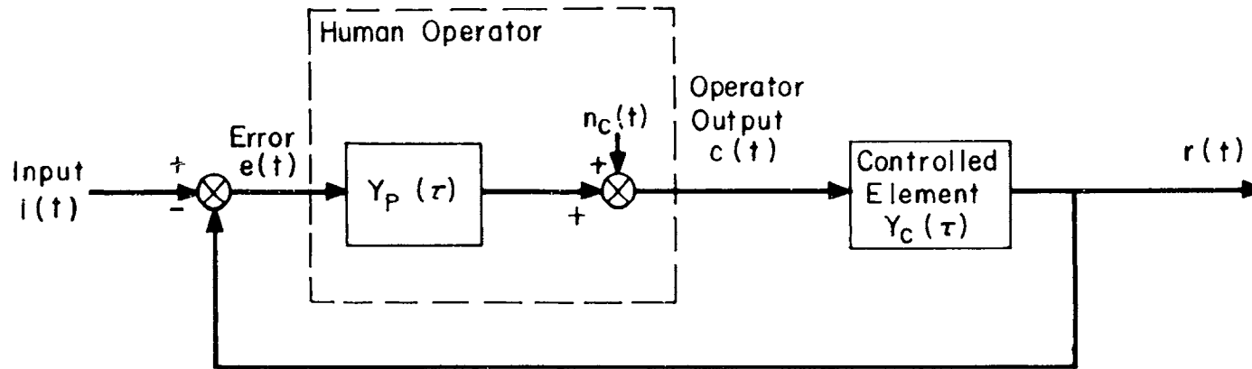
Fig.6.1 Block Diagram of Simple Compensatory Manual Control System (Ref. 129)
