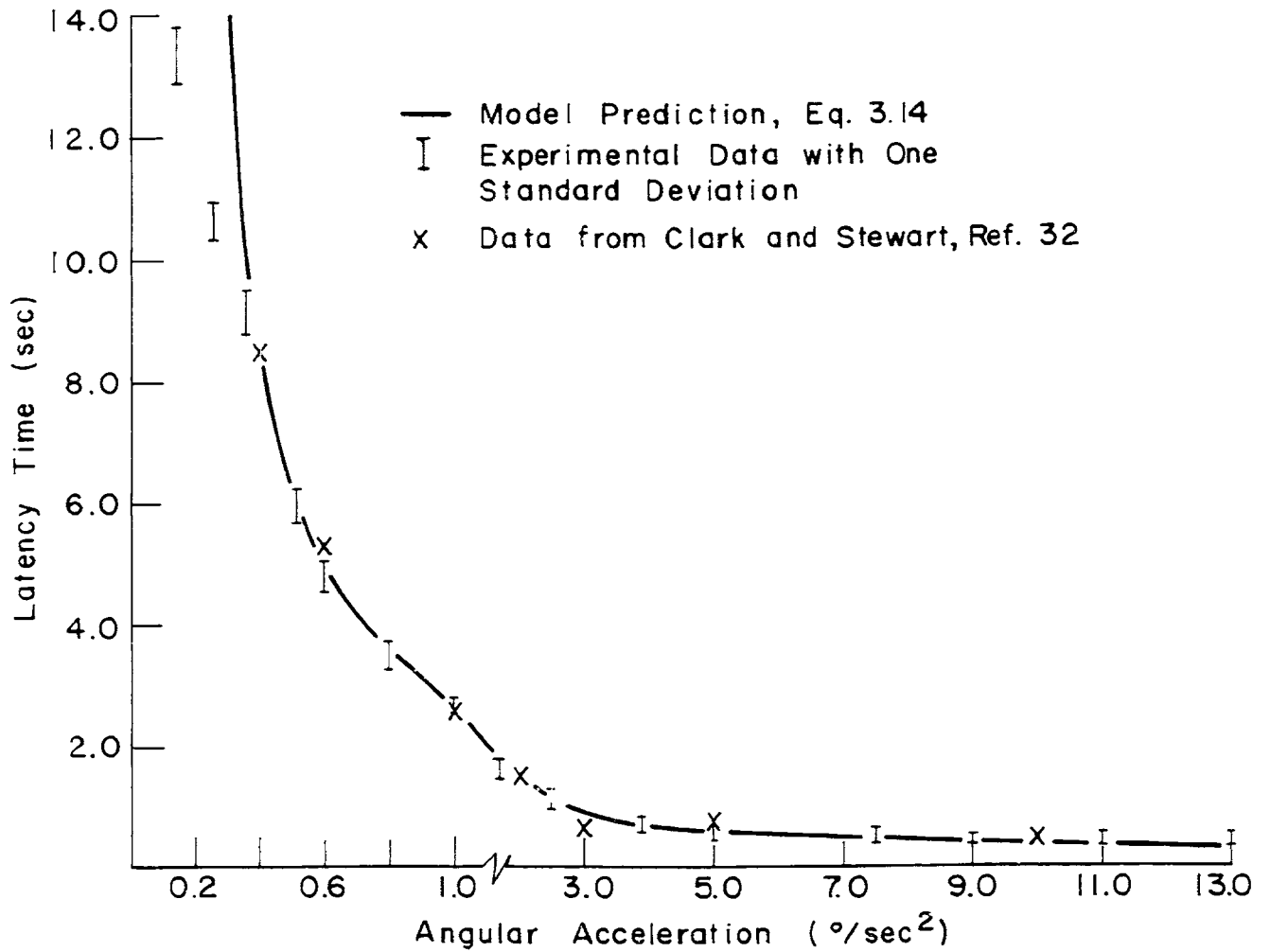
Fig. 3.4 Latency Times for Perception of Angular Acceleration about The Vertical Axis ( Y_h ) Note: Scale Change of Angular Acceleration
