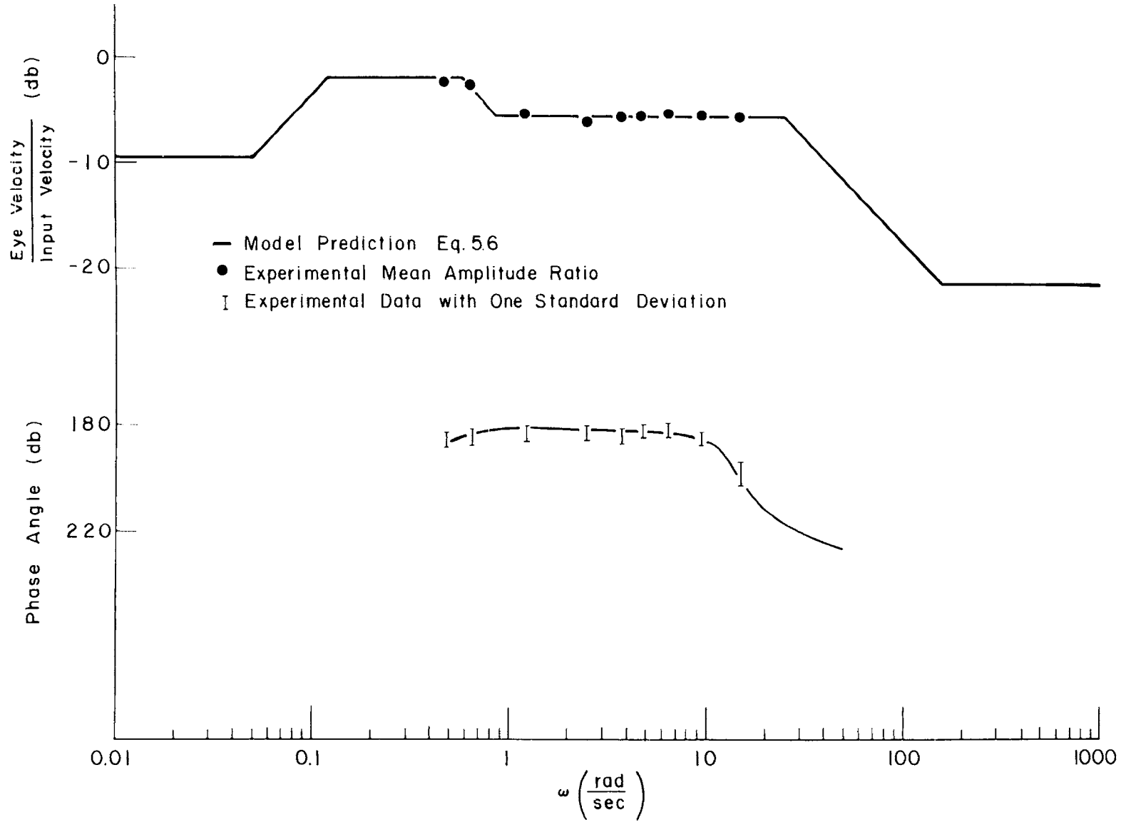
Fig. 5.12 Bode Plot of Compensatory Eye Movements (Vestibular and Neck Proprioception)
