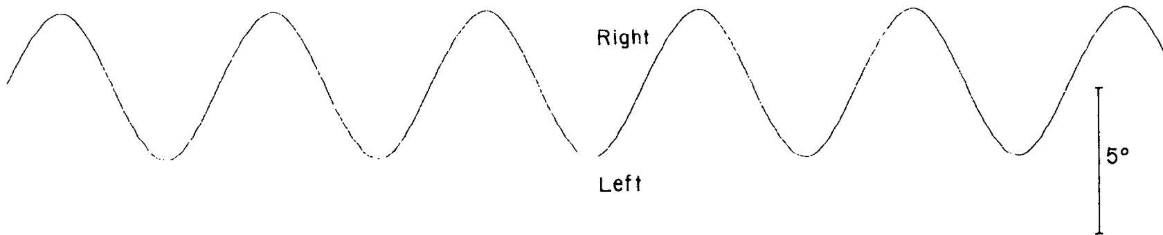
Fig. 5.6 Vestibular Compensatory Eye Movements With Earth-fixed Fixation Point, f = 1.0 cps
