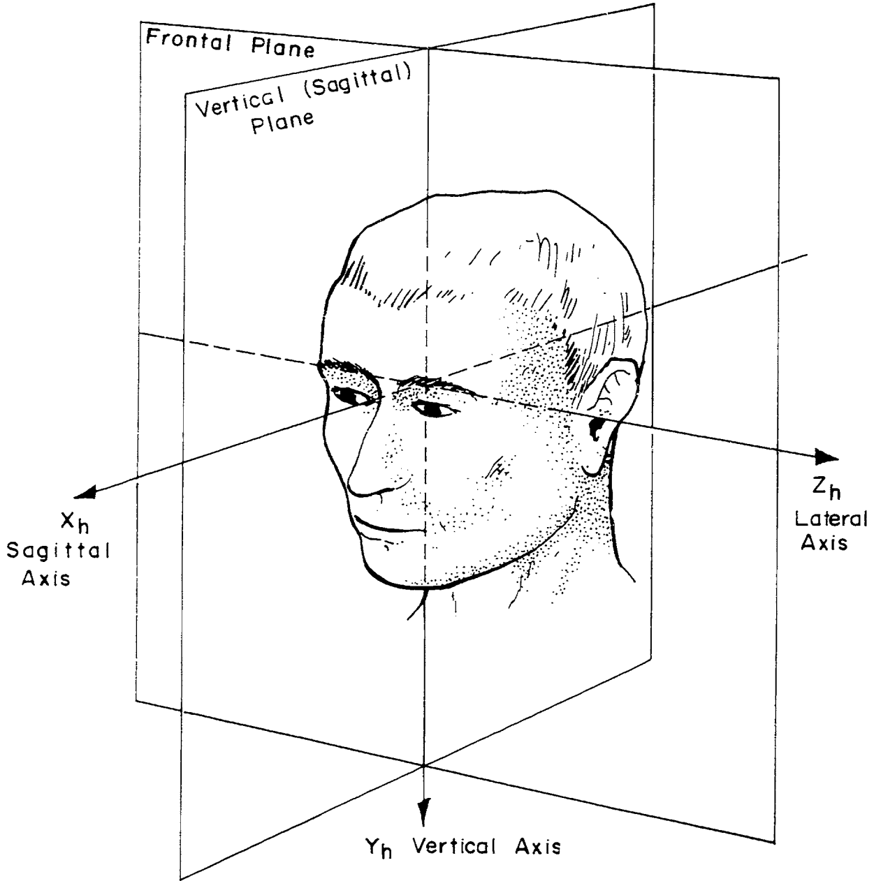
Fig. 2.4 The Head Planes and the Head Axis System
