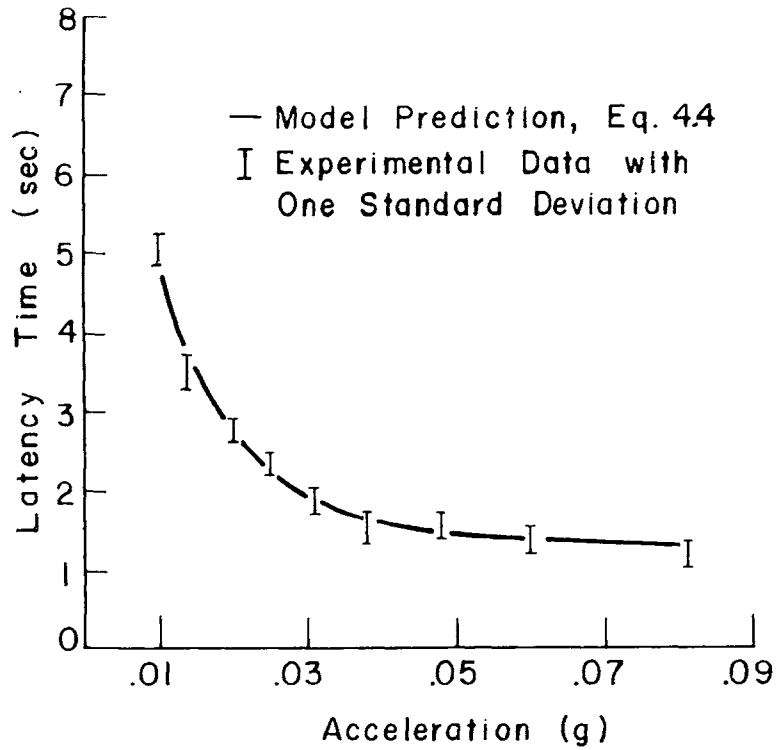
Fig. 4.5 Latency Times for Perception of Horizontal Linear Acceleration, Supine
