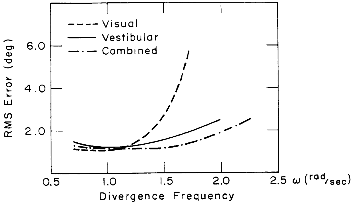
Fig. 7.7 RMS Error for Control of Inverted Pendulum
