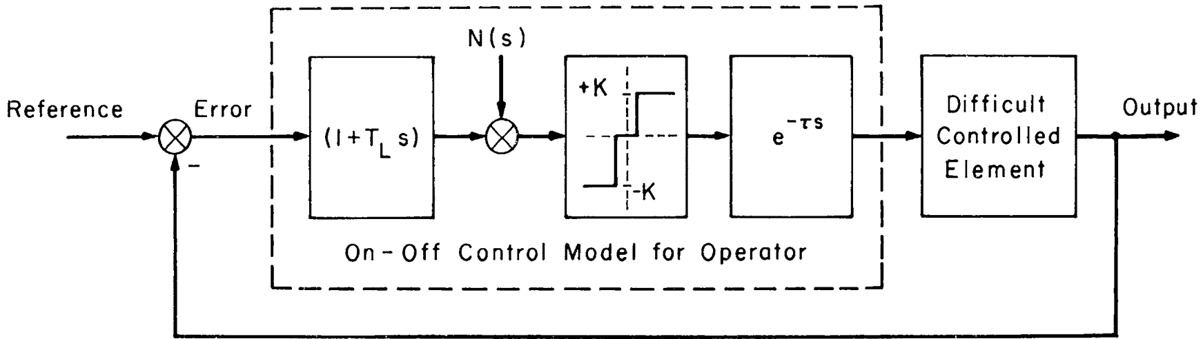
Fig. 7.3 Proposed On - Off Control Model for Human Operator in "Difficult" Control Task
