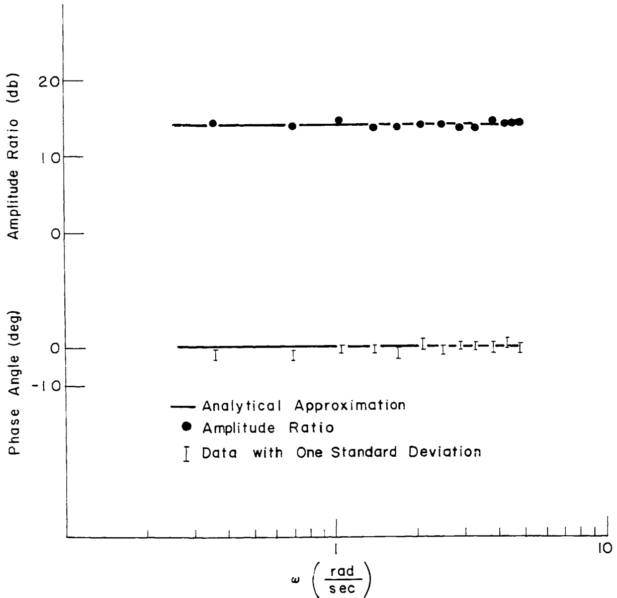
Fig. 6.4 Describing Function of the Human Operator in Motion Mode. Rotation with Respect to the Gravity Vector
