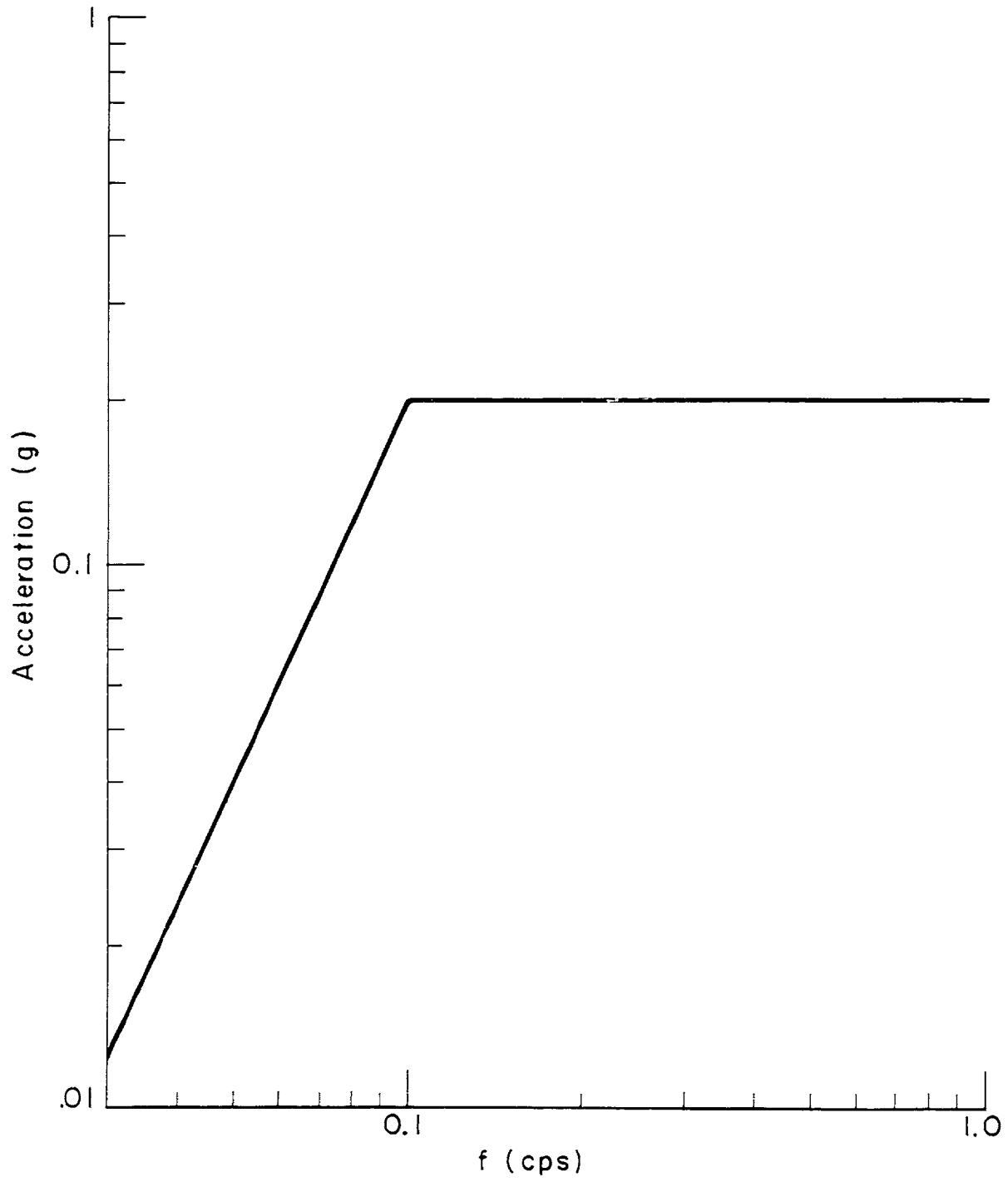
Fig. 4.2 Profile of Peak Sinusoidal Input Accelerations
