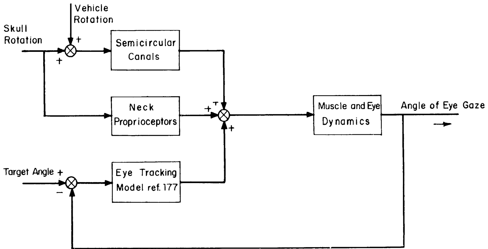
Fig. 5.1 Block Diagram of the Eye Movement Control System
