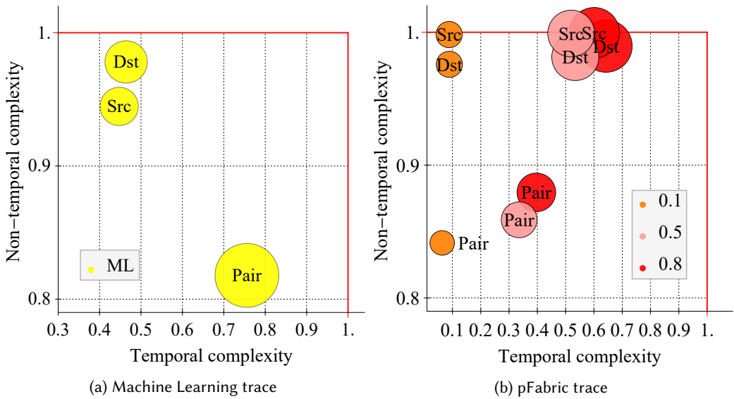
Fig. 7. Comparison of the complexity map of pair, source, and destination traces between (a) ML trace and (b) pFabric trace.
