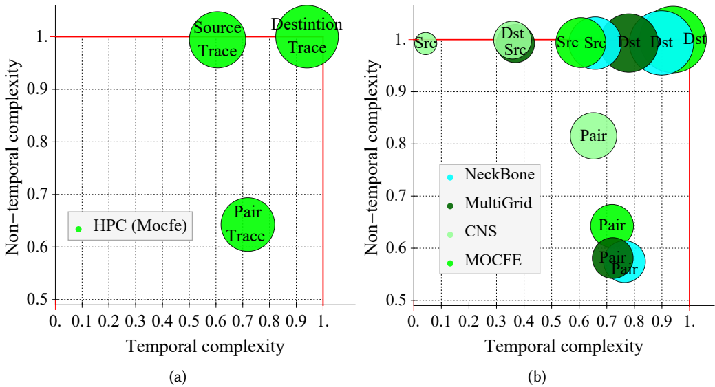
Fig. 6. HPC’s traffic complexity map. (a) A map of the MOCFE traffic trace. (b) The complexity map of four HPC traces with both pair and source/destination type traces.
