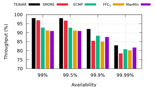
Figure 9: Averaged throughput guarantees for different \beta values on ATT, B4, and IBM topologies. TEAVAR is the only scheme that can explicitly optimize for a given \beta . For all the other schemes, the value on the x-axis is computed based on their achieved throughput.
