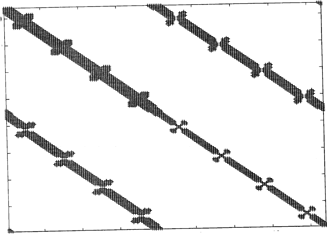
Figure 6-19: 168 \times 168 inverse estimation error covariance of state at \rho = 11 showing the entries greater than .01
