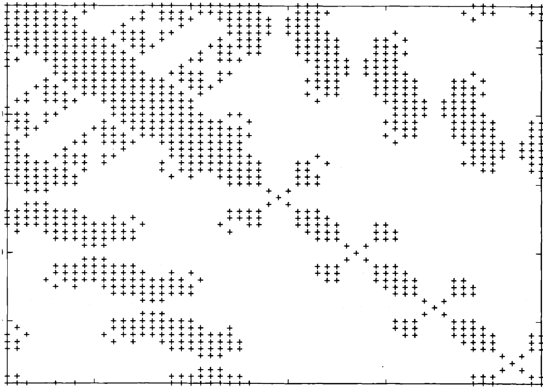
Figure 6-15: 56 \times 56 inverse estimation error covariance of state at \rho = 4 showing the entries greater than .01
