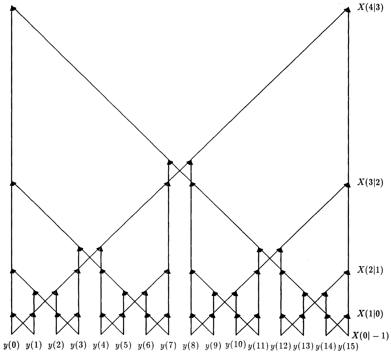
Figure 5-14: Parallel algorithm for 16 data points.
