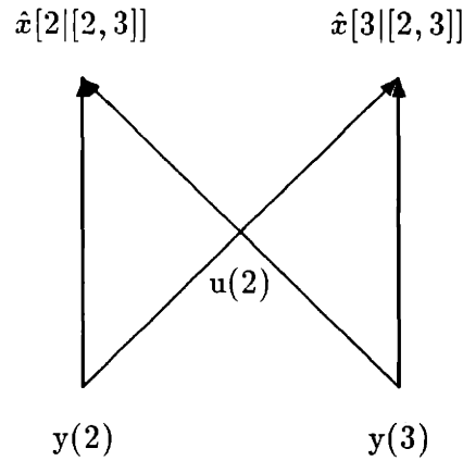
Figure 5-9: Computation of Processor #1
