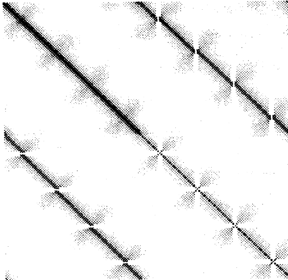
Figure 6-18: grayscale image of 168 \times 168 inverse estimation error covariance of state at \rho = 11
