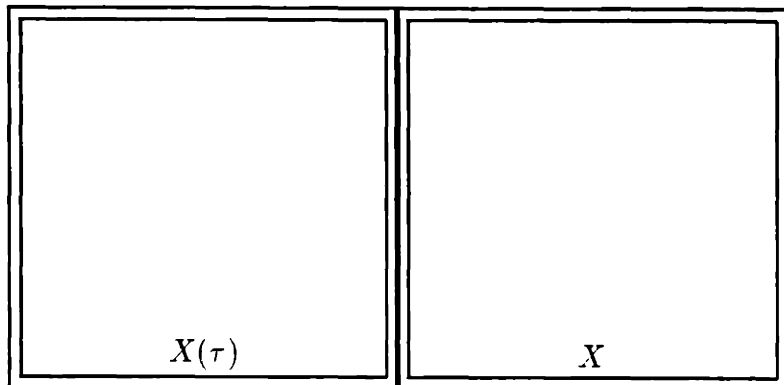
Figure 6-5: Two non-ordered 'states'
