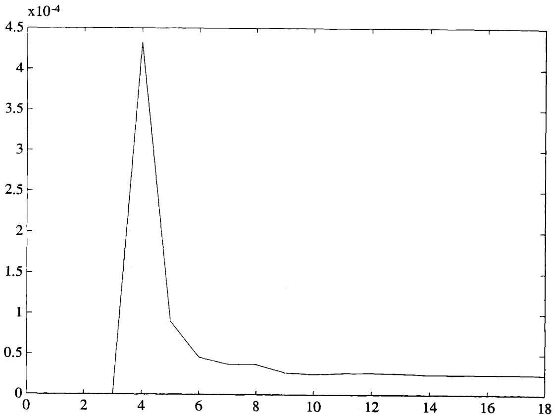
Figure 6-24: Maximum singular value plot for the difference between the optimal inverse estimation error covariance of the optimal filter and the actual inverse estimation error covariance for the suboptimal filter. The minimum singular value for the optimal inverse estimation error covariance is equal to 1.
