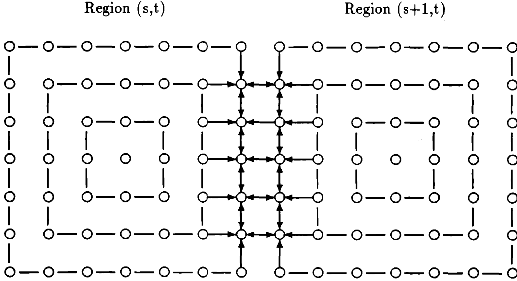
Figure 6-9: Two neighboring regions for the Measurement Update step and the dynamic constraints (which are shown by the arrows) required to merge them.
