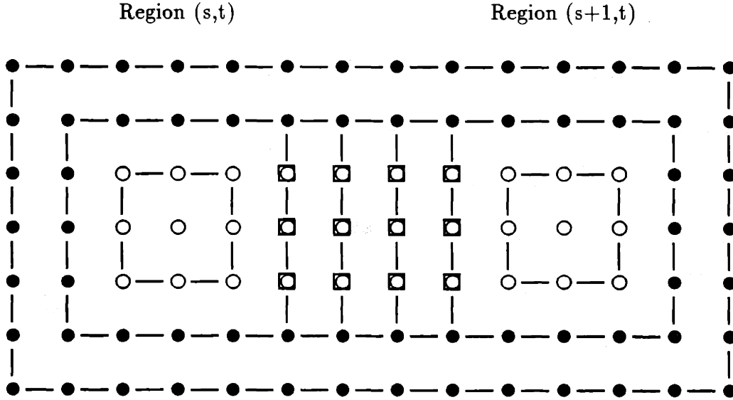
Figure 6-10: Constructing the boundary enclosing two regions from the boundaries of two subregions X(s,t) and X(s+1,t) . The black dots represent the boundary which encloses both regions which will be denoted by X(\{s,s+1\},t) . The twelve dots which are enclosed by squares are the elements of \Upsilon(\{s,s+1\},t) . \Upsilon(\{s,s+1\},t) are elements of the union of X(s,t) and X(s+1,t) but are not elements of X(\{s,s+1\},t) .
