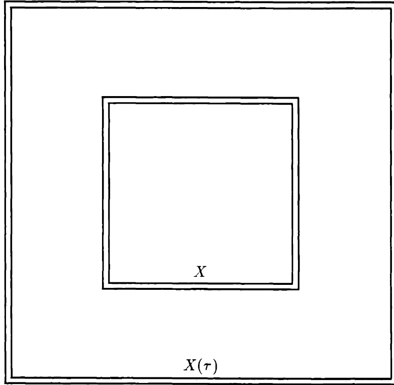
Figure 6-4: Two ordered 'states'
