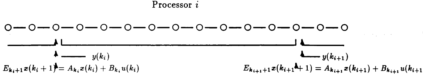
Figure 5-1: partitioning of the data among processors
