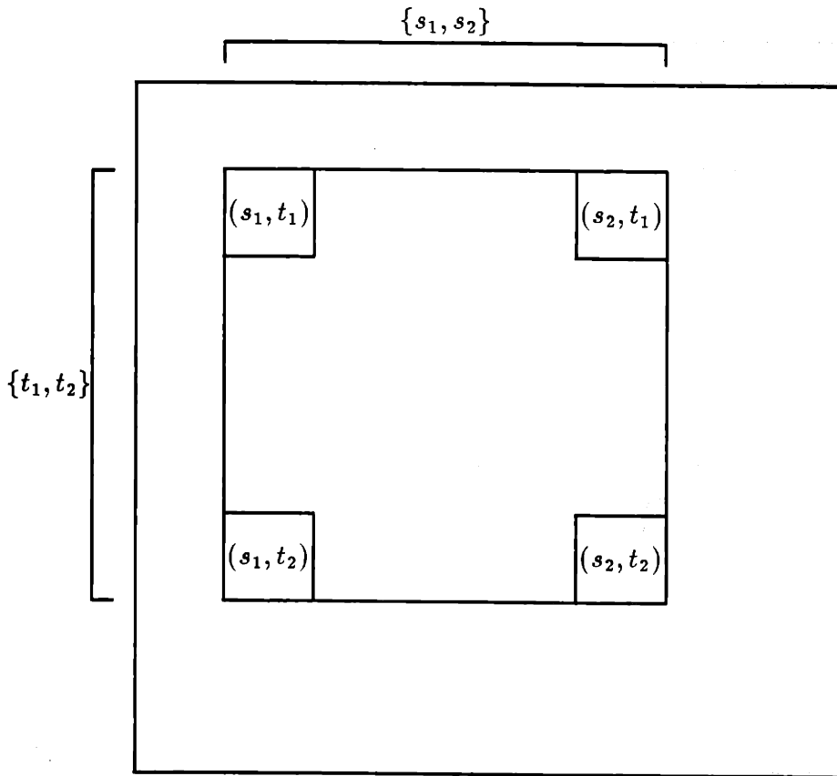
Figure 6-7: The notation (\{s_1, s_2\}, \{t_1, t_2\}) is used to refer to rectangles constructed from the union of individual square regions. Similarly the boundary for this region is denoted by X(\{s_1, s_2\}, \{t_1, t_2\})
