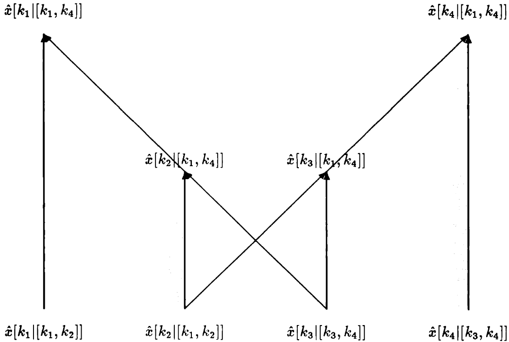
Figure 5-10: Using estimates of x(k_2) and x(k_3) to update x(k_1) and x(k_4) where k_3 = k_2 + 1 . Specifically, the estimates \hat{x}[k_2|[k_1, k_2]] , and \hat{x}[k_3|[k_3, k_4]] are combined to produce the estimate of x(k_2) and x(k_3) given all of the data denoted by \hat{x}[k_2|[k_1, k_4]] and \hat{x}[k_3|[k_1, k_4]] respectively. The correlation between the estimation errors \tilde{x}[k_1|[k_1, k_2]] , and \tilde{x}[k_2|[k_1, k_4]] is then used to update \hat{x}[k_1|[k_1, k_4]] to the smoothed value given by \hat{x}[k_1|[k_1, k_4]] . This represents the basic building block for the algorithm in this section.
