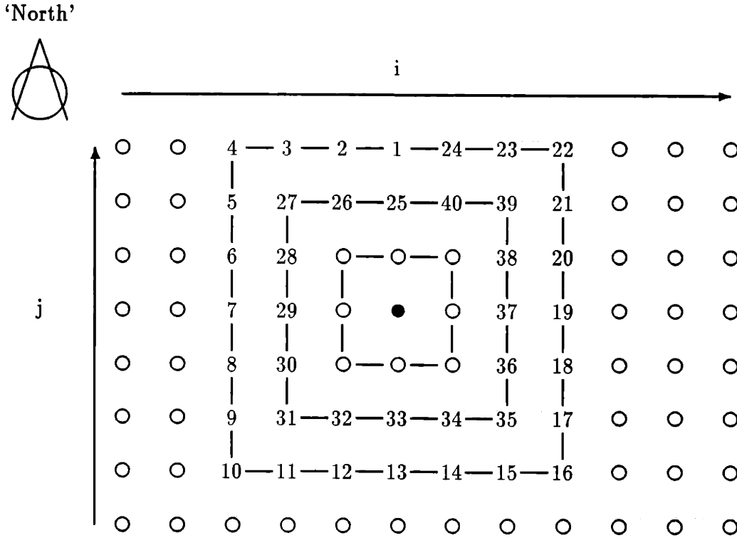
Figure 6-8: The integer function \Theta(i, j, 3) . The shaded dot is the origin, (i, j) = (0, 0) . This function orders the elements x(i, j) in the vector X(\rho) .
