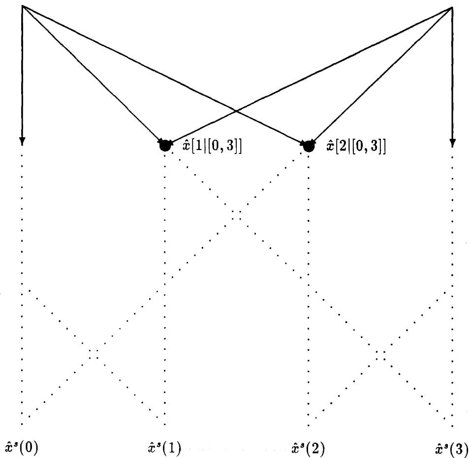
Figure 5-12: Additional boundary information in the form of the smoothed estimates \hat{x}^s(0) and \hat{x}^s(3) are combined with two estimates \hat{x}[1|[0,3]] and \hat{x}[2|[0,3]] , which are represented by the large dots, to produce the smoothed estimates \hat{x}^s(1) and \hat{x}^s(2) . The dotted lined indicate the flow of data which was used to construct the estimates \hat{x}[1|[0,3]] and \hat{x}[2|[0,3]] . The additional boundary information can be obtained by viewing the figure to be a part of an algorithm operating on a larger set of data as in Figure 5-13
