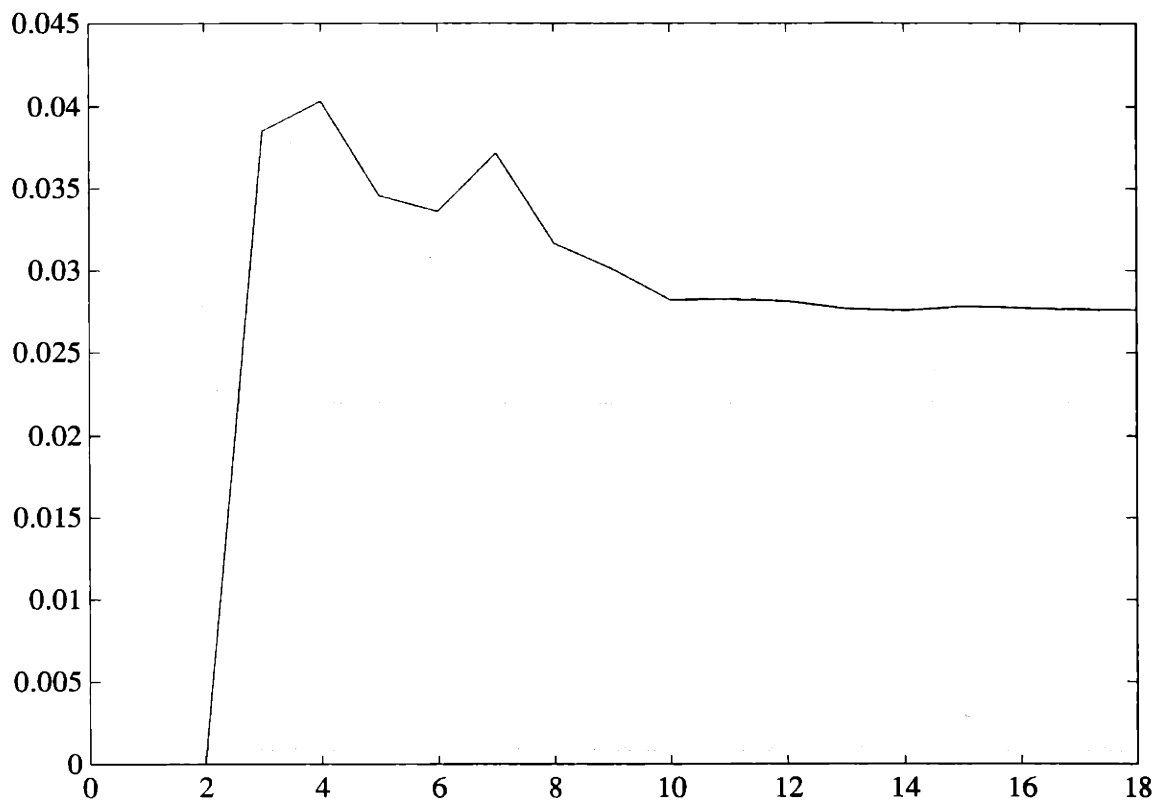
Figure 6-20: Maximum singular value plot for the difference between inverse estimation error covariance for the state at different radii and the approximation to that inverse estimation error covariance based on setting values smaller than .01 to 0. Plot starts at \rho = 2 .
