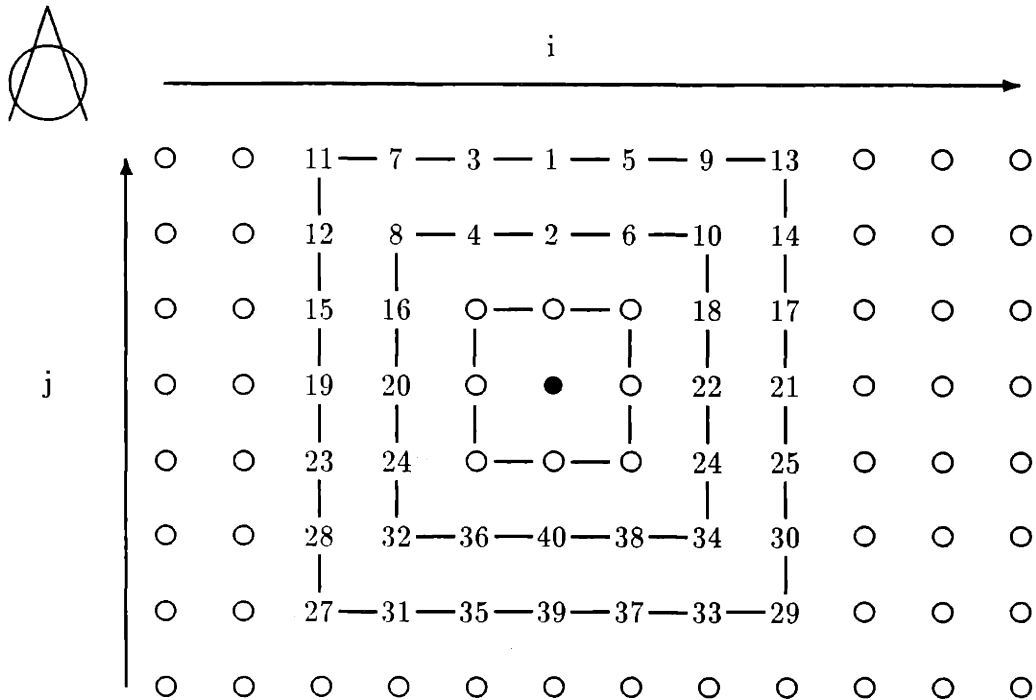
Figure 6-21: The integer function \Theta as a function of i and j for \rho = 3 . Here the elements are ordered so that we may perform our processing moving outward from the center of one leg and eventually terminate moving inward on the opposite leg of the square boundary.
