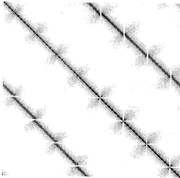
Figure 6-16: grayscale image of 168 \times 168 estimation error covariance of state at \rho = 11
