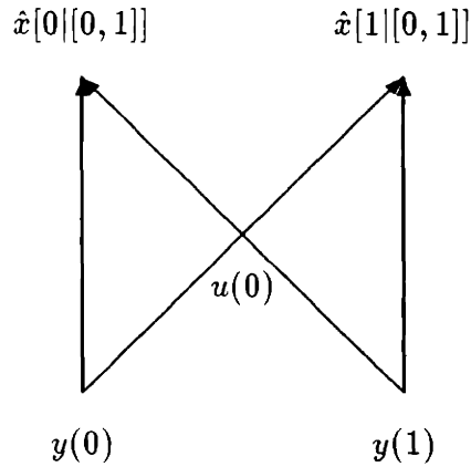
Figure 5-8: Icon representing the combining of two neighboring estimates using the dynamic constraint which links them
