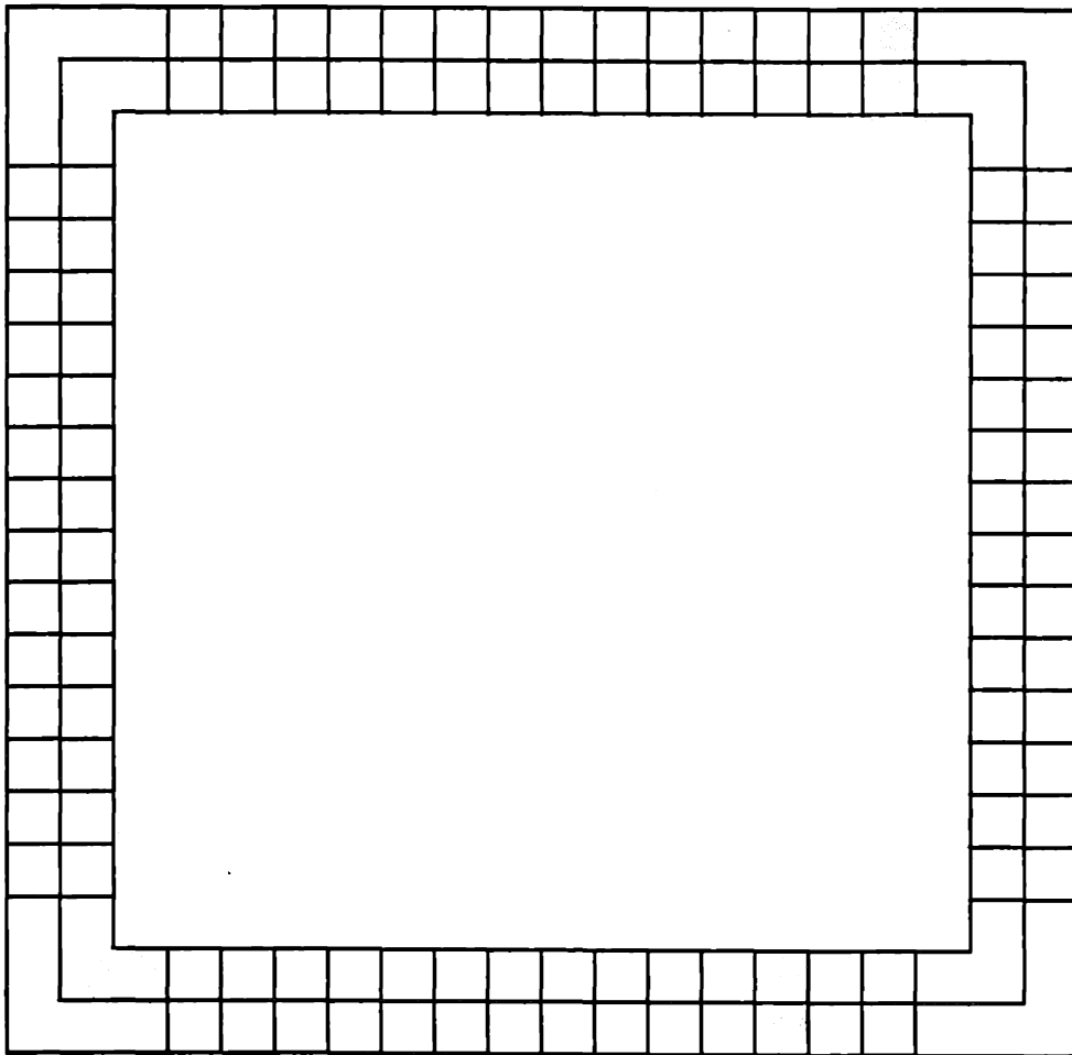
Figure 6-26: Partitioning the state X(\rho + 1) so that it agrees with the partitioning of X(\rho)
