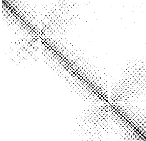
Figure 6-22: The inverse estimation error covariance at \rho = 11 after the elements have been reordered. Large elements of the matrix have been moved to locations near the main diagonal.
