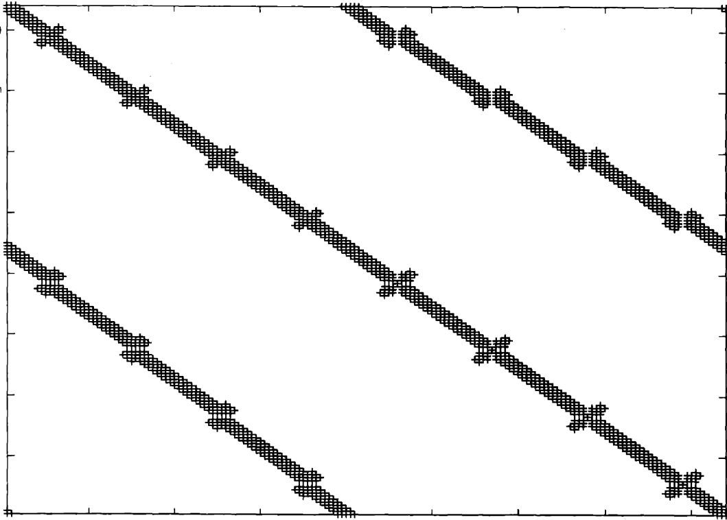
Figure 6-17: 168 \times 168 estimation error covariance of state at \rho = 11 showing the entries greater than .01
