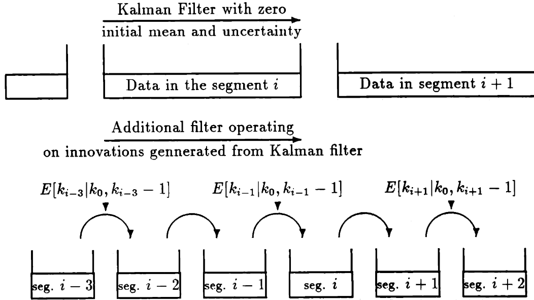
Figure 5-2: Parallel estimation in algorithm by Morf et al.
