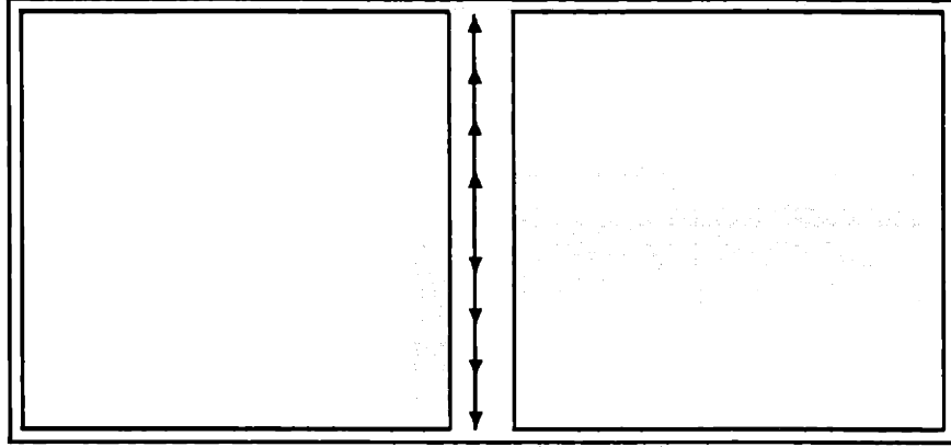
Figure 6-23: Filtering outward along a common boundary
