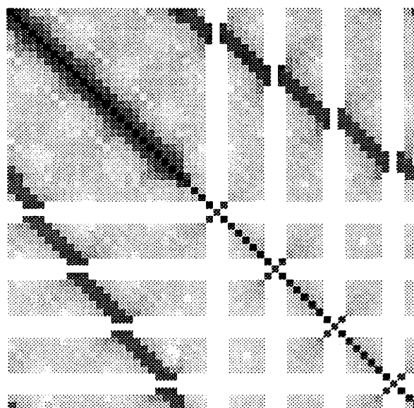
Figure 6-14: grayscale image of 56 \times 56 inverse estimation error covariance of state at \rho = 4
