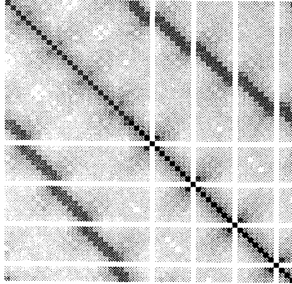
Figure 6-12: grayscale image of 56 \times 56 estimation error covariance of state at \rho = 4 N = S = E = W = B = 1 with observations given by
