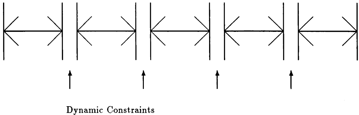
Figure 5-4: This represents the system immediately after the local filtering which starts at the center of each subinterval and ends at the boundary of each subinterval has been performed. The the state of the system has dimension 2n , and the local estimates produced by each processor represents local estimates of the state. Linking the states together are the remaining constraints. If neighboring states do not intersect then the constraints are noisy and are a subset of the of the original set of descriptor equations (5.1). Otherwise neighboring states intersect and equality constraints exist (??)
