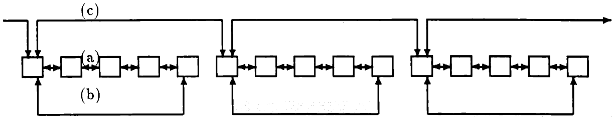
Figure 5-7: Each processor in the parallel algorithm in Section 5.5 produced boundary measurements for its region which are communicated to neighboring processors. Each block represents a processor operating on a specified region and local boundary measurements are communicated to neighboring processors using communication links such as the one indicated by (a). In order to gain greater efficiencies local regions can be grouped in clusters where one processor is responsible for obtaining the boundary measurement for the entire region covered by a cluster of processors. This processor can obtain this information from communication links (a), and (b). Finally all processors which are responsible for obtaining the boundary information from a cluster of processors can then communicate among themselves to produce the optimal boundary estimate for each cluster. Then each cluster in parallel can work to disseminate the optimal cluster boundary information to produce optimal estimates of local boundaries. Finally the optimal boundary information of each local boundary can be used by each processor in parallel to update interior points of each subregion.
