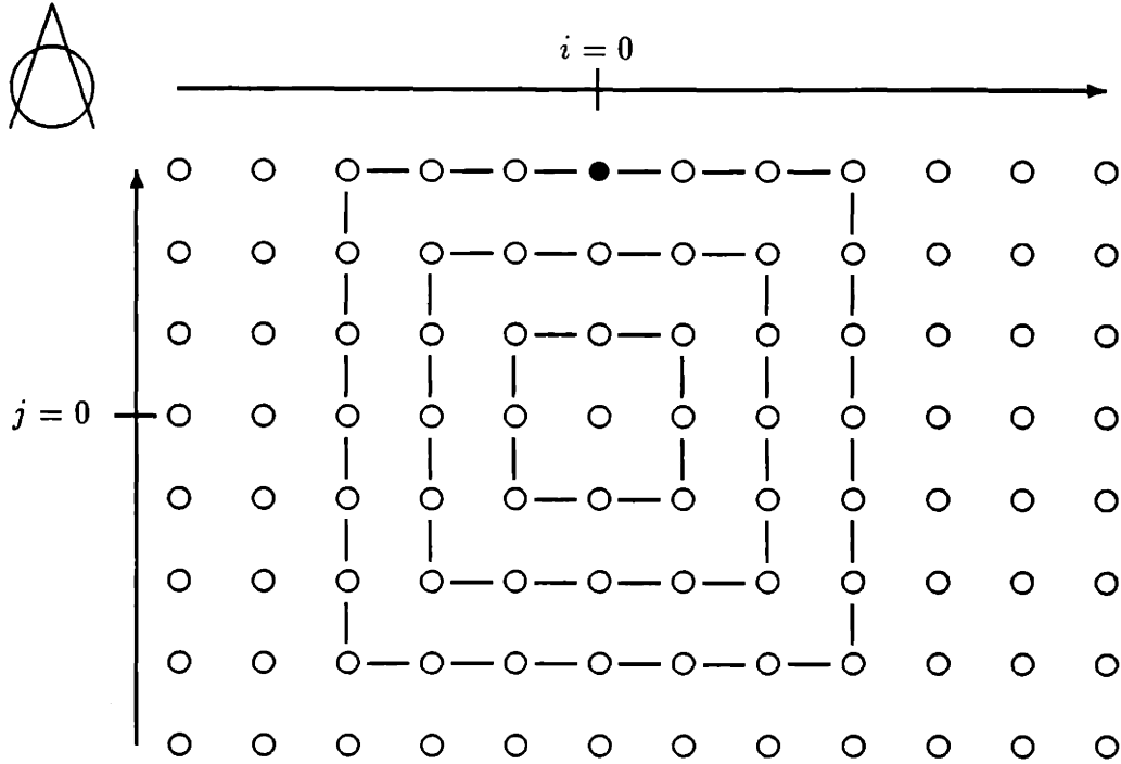
Figure 6-3: Square ordering of the elements of \chi_\mu(\rho) . \rho \in \{0, 1, 2, 3\} , \mu = \infty
