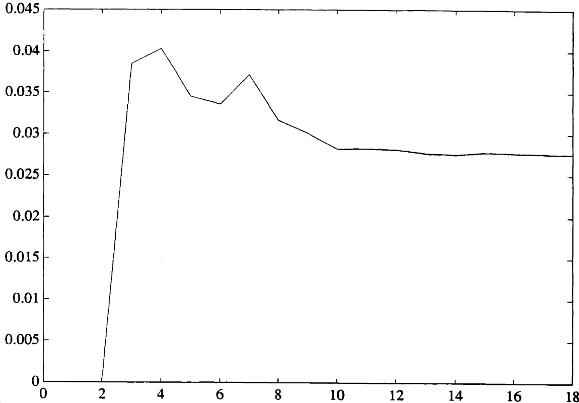
Figure 6-25: Maximum singular value plot of approximated inverse estimation error covariance to the optimal inverse estimation error covariance
