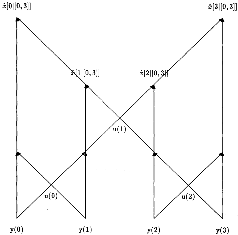
Figure 5-11: Arriving at the smoothed estimate for the boundary of the entire region estimation algorithms.
