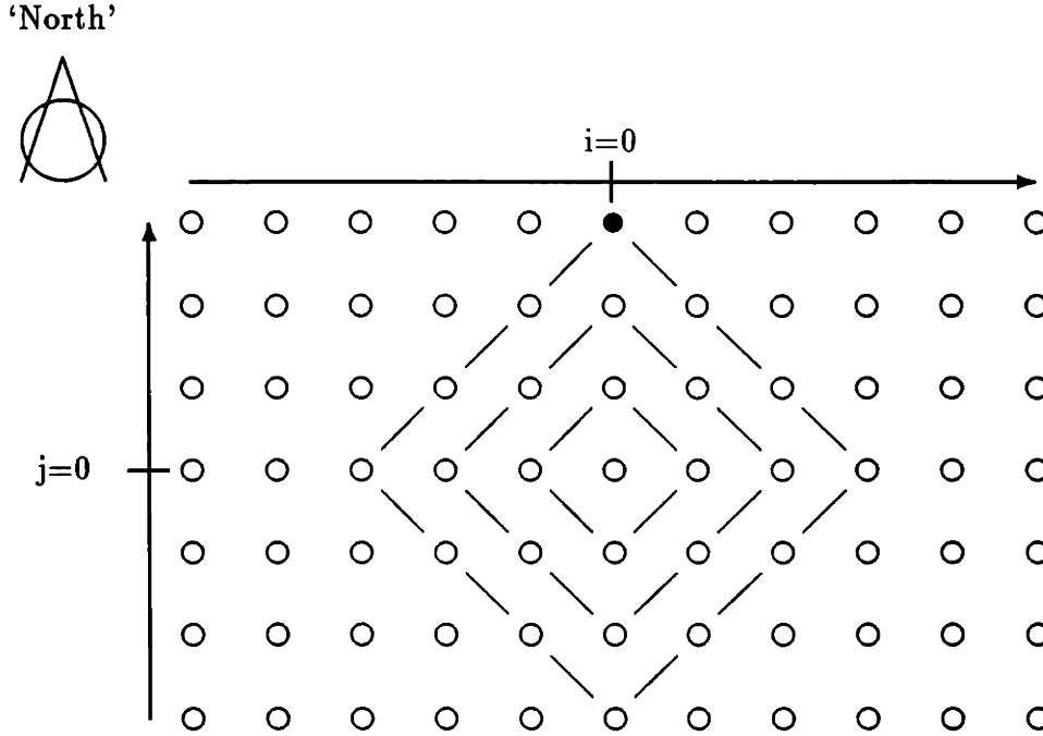
Figure 6-2: Diamond ordering of the elements in \chi_\mu(\rho) . \rho \in \{0, 1, 2, 3\} , \mu = 1
