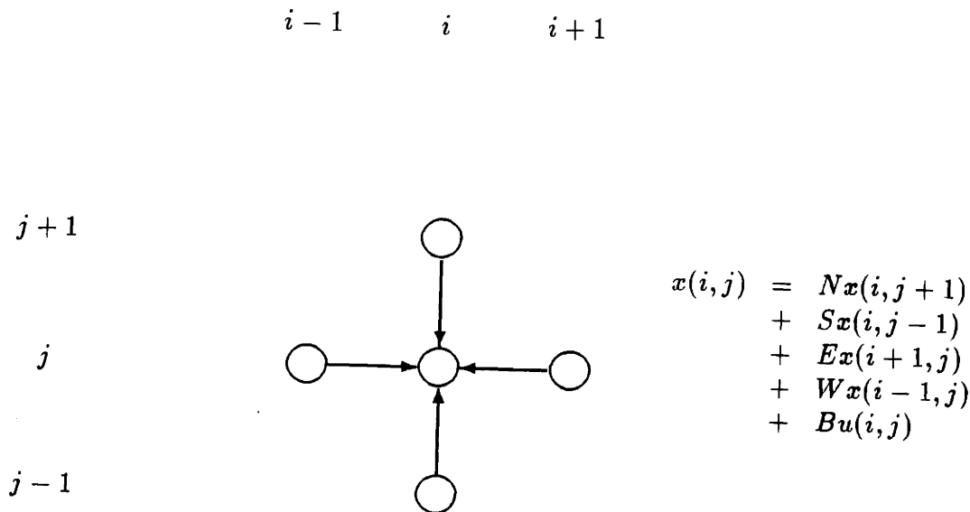
Figure 6-1: Nearest Neighbor Dependency
