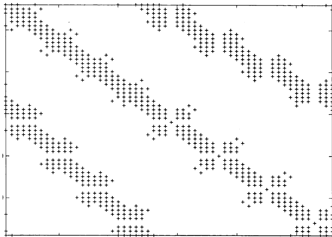
Figure 6-13: 56 \times 56 estimation error covariance of state at \rho = 4 showing the entries greater than .01
