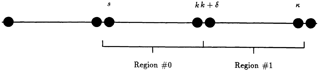
Figure 5-15: The dots represent the boundary of neighboring regions which will be merged together in the measurement update step. Region #0 and Region #1 will be merged together in into a region bounded by the points s and \kappa .
