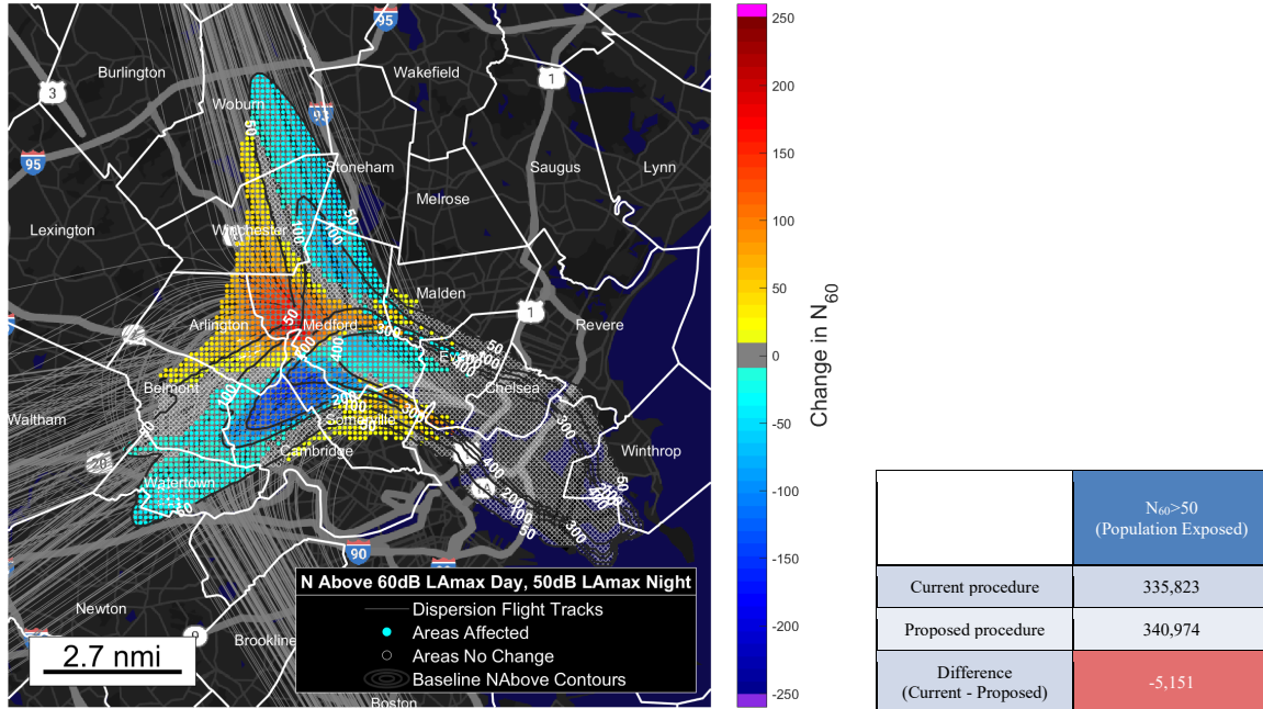
Figure 36. Noise results for Runway 33L Altitude-Based Dispersion at 3000 ft.
