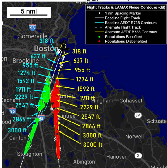
Figure 23. 4R RNP approach with 24-degree intercept.
