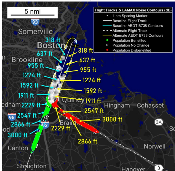
Figure 22. 4R RNAV Route 3 Initial Approach.
