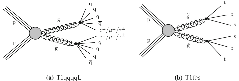
Fig. 3 Diagrams illustrating the two simplified RPV SUSY models considered in this analysis
