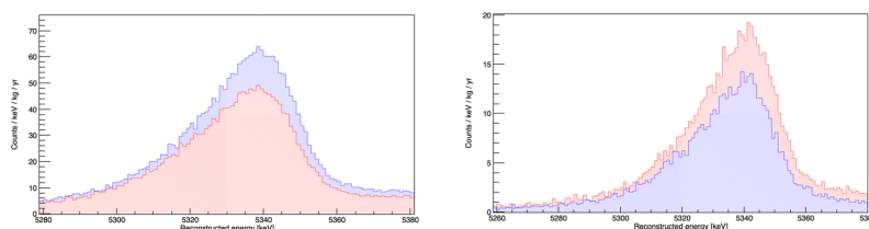
Fig. 7 M_1 ( left ) and M_2 ( right ) spectrum comparison in the region of the \alpha particle from ^{210}\text{Po} decay. Histograms in blue ( red ) are referred to derivative (optimum) trigger analysis. (Color figure online)
