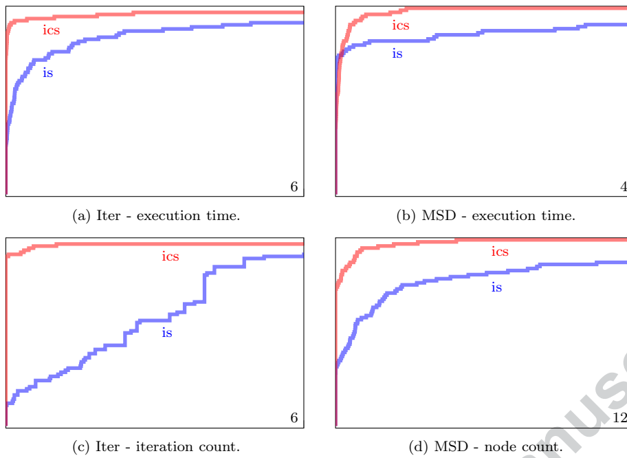
Fig. 6: \mathcal{K}^* cut types performance profiles.
