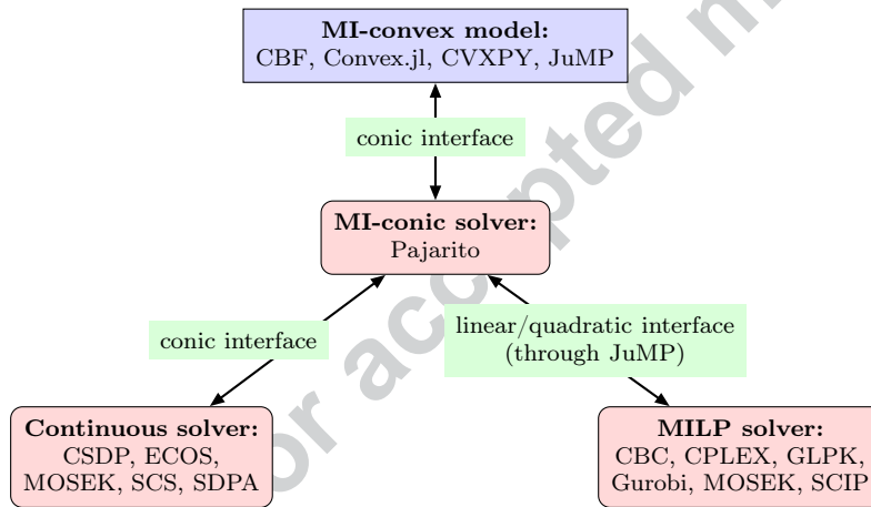
Fig. 1: Pajarito’s integration with MathProgBase.
