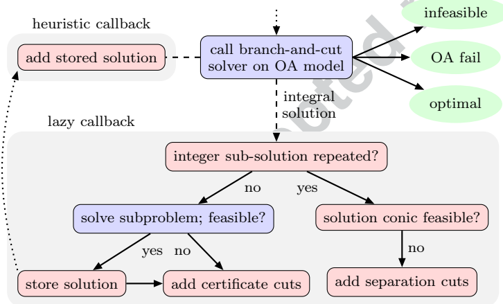
Fig. 4: Pajarito’s MIP-solver-driven (MSD) method, following initialization.
