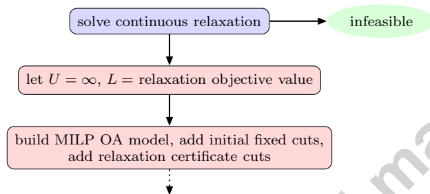
Fig. 2: Pajarito's OA model initialization.
