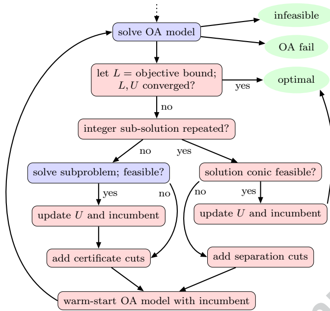
Fig. 3: Pajarito’s iterative method, following initialization.
