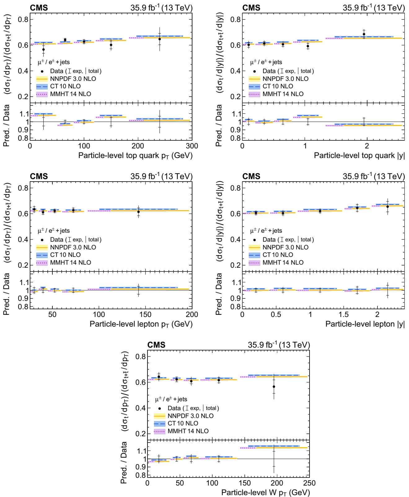
Fig. 12 Ratio of the top quark to the sum of the top quark and anti-quark t -channel differential cross section at the particle level: (upper row) top quark p_T and rapidity; (middle row) charged lepton p_T and rapidity; (lower row) W boson p_T . The total uncertainty is indicated by the vertical lines, while horizontal bars indicate the statistical and
