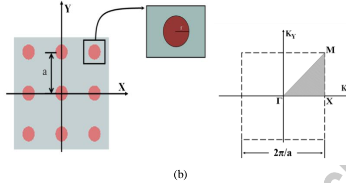
Fig.2. Proposed structure of PhC based single MRR: (a). Perspective view, (b). Front view
