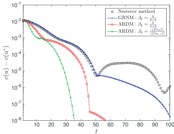
FIG. 5. Convergence of the error in the objective value c(\mathbf{u}) = 0.02u_1^2 + 0.005u_2^2 for Nesterov's method, the gradient restarting Nesterov method (GRNM), and the ARDM with \beta = k/(k+3) and \beta_k = \|\mathbf{f}(\mathbf{u}_k)\|/\|\mathbf{f}(\mathbf{u}_{k-1})\| .
