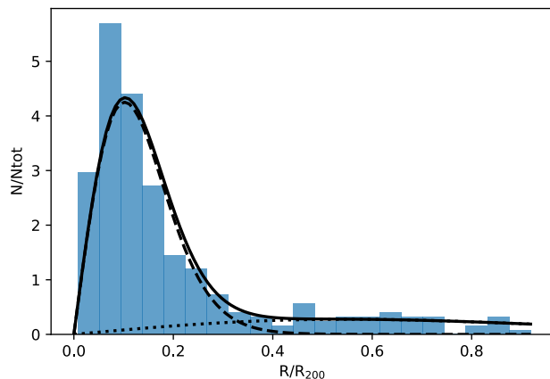
Figure 2. Normalized histogram of the BCG-SZ offset distribution. The D_{\text{BCG-SZ}} distribution can be described as the sum (black line) of a relaxed distribution (dashed line) plus a disturbed distribution (dotted line). The disturbed sample consists of the clusters with R > 0.4 \times r_{200} and D_{\text{BCG-SZ}} > 3\Delta\theta .
