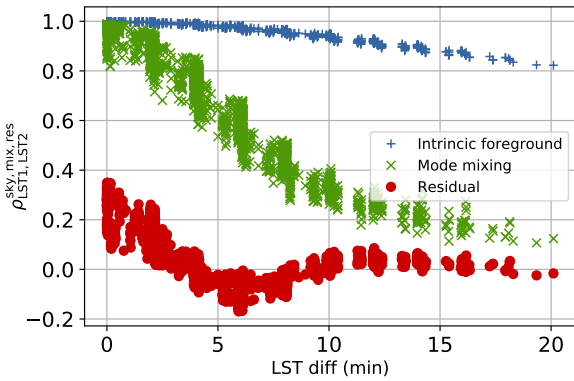
Figure 10. Correlation coefficient \rho_{LST1,LST2}^{\text{sky,mix,res}} as a function of LST difference for all the night, LST-binned data. Each marker symbol ('+', 'x' or 'o') represents an LST difference.
