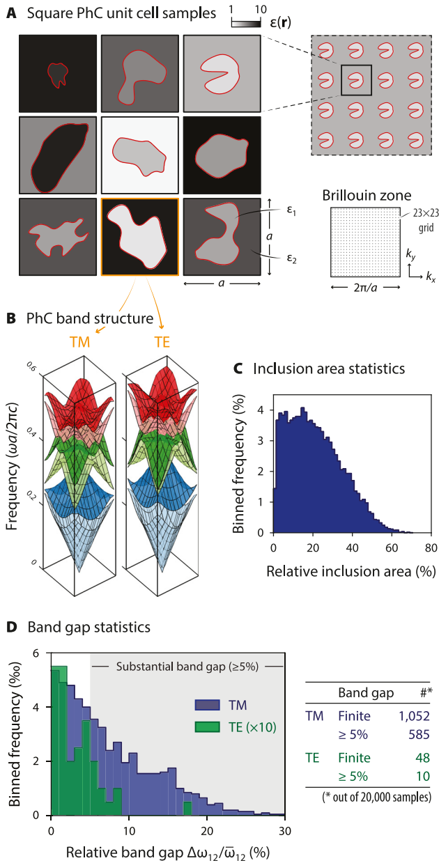
Figure 1: Photonic crystal data set. We generated a data set of 20,000 square 2D PhC unit cells, each consisting of a smooth, centered inclusion of permittivity \epsilon_1 in a background permittivity \epsilon_2 with \epsilon_i \in [1, 10] . (A) Several representative unit cells and the BZ grid-sampling used in the calculation of band structures. (B) The TM and TE band structures of the PhC highlighted in orange in (A). (C) The generated unit cells predominately feature inclusions occupying less than half the unit cell, as illustrated by a histogramming of the relative inclusion areas across the data set. (D) TM band gaps between bands 1 and 2 consequently occur much more frequently than TE gaps, as TE gaps mainly arise in “filamentary” networks, corresponding to large relative inclusion areas.
