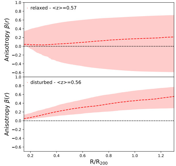
Figure 9. Velocity anisotropy profile \beta(r) recovered when separately analyzing relaxed and un-relaxed clusters. For the latter, the anisotropy profile indicates that the galaxies in the clusters are moving on nearly isotropic orbits near the center and increasingly radial orbits out toward the virial radius R_{200} . The recovered anisotropy profile for the relaxed clusters is consistent with these results, but exhibits much larger uncertainties that allow for a much broader range of galaxy orbits.
