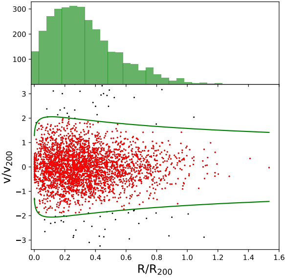
Figure 3. The projected phase-space diagram (below) in the rescaled coordinates (R/R_{200}, v/v_{200}) for the full sample. Green lines represent the radially-dependent 2.7\sigma_{\text{LOS}} cut used to reject interlopers (indicated by black dots). The radial distribution of the member galaxies with measured redshifts is shown in the upper panel.
