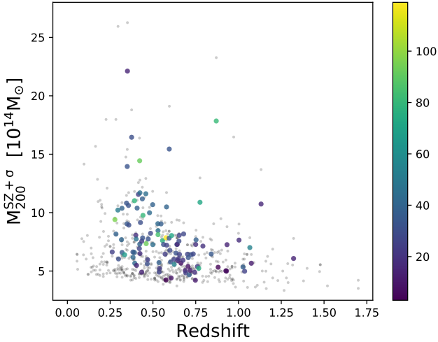
Figure 1. Masses vs redshifts of the cluster sample. The colored dots are coded according to the number of member galaxies in each cluster (see color bar on right). Overplotted in grey is the full distribution of the 2500 deg 2 SPT-SZ sample.
