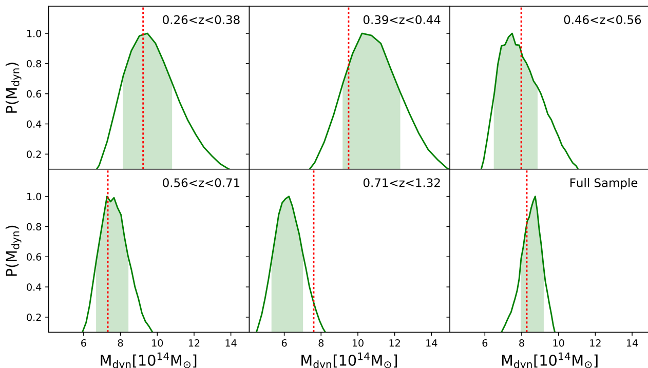
Figure 7. Marginalized distribution of the dynamical masses. Each panel corresponds to a different redshift range, and the final panel shows the results of the analysis of the full sample. In green we highlight the 1\sigma confidence region. The red line represents the mean SPT+ \sigma mass \langle M_{200}^{\text{SZ}+\sigma} \rangle for the clusters in the bin, weighted by the number of member galaxies in the individual clusters. There is a good agreement between the dynamical masses and the originally inferred SPT masses in all cases (see Table 6).
