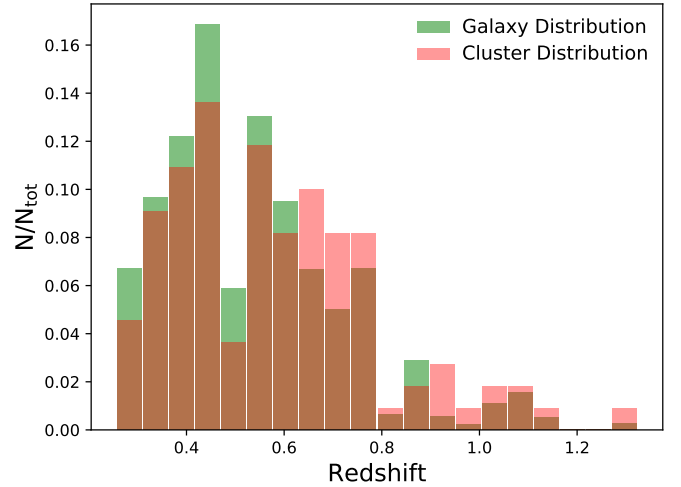
Figure 2. Redshift distribution of member galaxies (green) and clusters (red) in our sample, normalized to the total number of objects in each case. The two distributions are similar, but a clear trend to have fewer galaxies per cluster at high redshift is visible.
