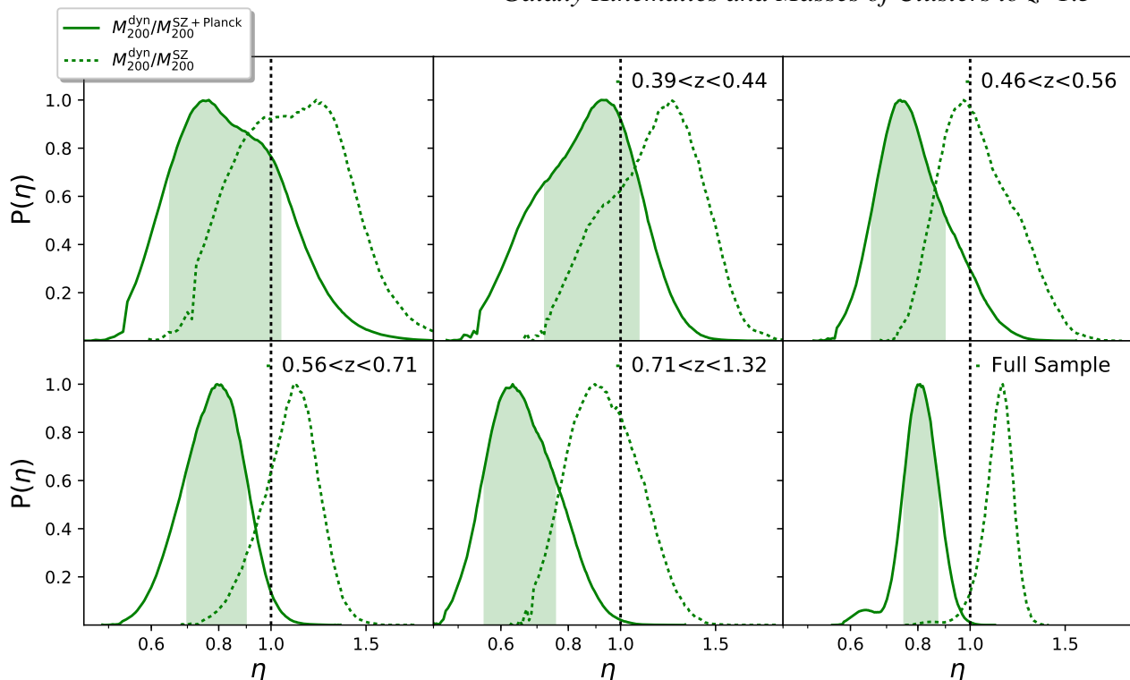
Figure 8. Posterior distribution of \eta = M_{200}^{\text{dyn}}/M_{200}^{\text{SZ+Planck}} (solid green lines) arising from a dynamical analysis of each cluster subsample. The green region shows the 1\sigma region, while the vertical dotted black line marks the value \eta = 1 . These distributions show that in the two high redshift bins and for the full sample there is disagreement between the dynamical masses and the SPT+Planck calibrated cluster masses. For the full sample the discrepancy is 1.9\sigma significant when including estimates of the systematic uncertainties. In the highest redshift bin, the discrepancy is 2.6\sigma . The dashed green lines show the estimated posterior for \eta' = M_{200}^{\text{dyn}}/M_{200}^{\text{SZ}} , where M_{200}^{\text{SZ}} represents the de Haan et al. (2016) masses calibrated using the SPT mass function and Y_X measurements for many of the systems. In contrast to the SPT+Planck masses, these masses are in good agreement ( 1\sigma offset) with the dynamical masses.
