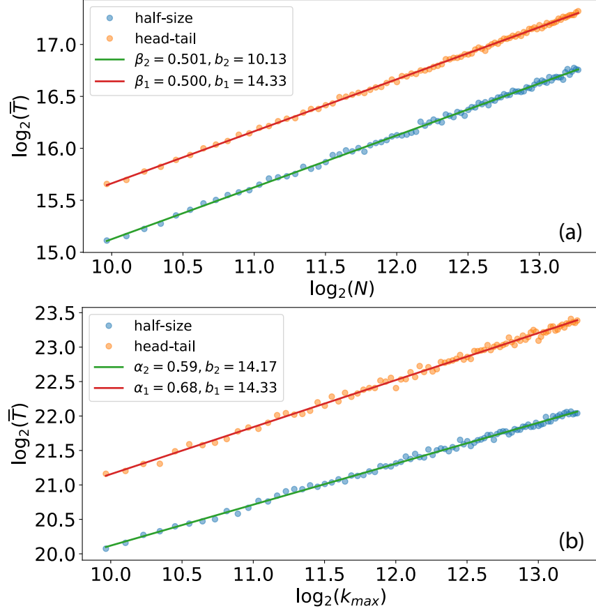
FIG. 1: (color online) Scaling behavior of ensemble averaged running time \bar{T} as a function of N and k_{\max} . For a given N and k_{\max} , we uniformly sample k_{\text{true}} \in [0, k_{\max}] 300 times. For each k sample, we follow the predictive dissonance protocol to pinpoint k and record the running time T , and we choose repetition J = 6 . The ensemble averaged time \bar{T} is plotted for each N and k_{\max} . In subplot (a), it shows \bar{T} \propto N^\beta , where \beta is approximately 0.5; in subplot (b), it shows \bar{T} \propto k_{\max}^\alpha , and \alpha depends on the details of pairing schemes.
