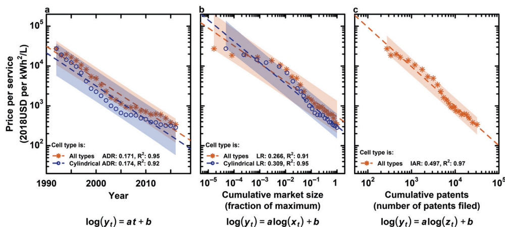
Fig. 10 Lithium-ion price per service regressed against a variety of possible determinants. Lithium-ion cell price per service (in \text{kWh}^2 \text{h}^2 \text{L}^{-1} ) regressed against year (a), cumulative market size (b), and cumulative patent filings (c) for all (orange asterisk marks) and cylindrical (blue circles) cells. Prediction intervals (95% level) are plotted as similarly colored shaded regions. Analyses are restricted to the years 1992 through 2016, and market size is measured in number of cells.
