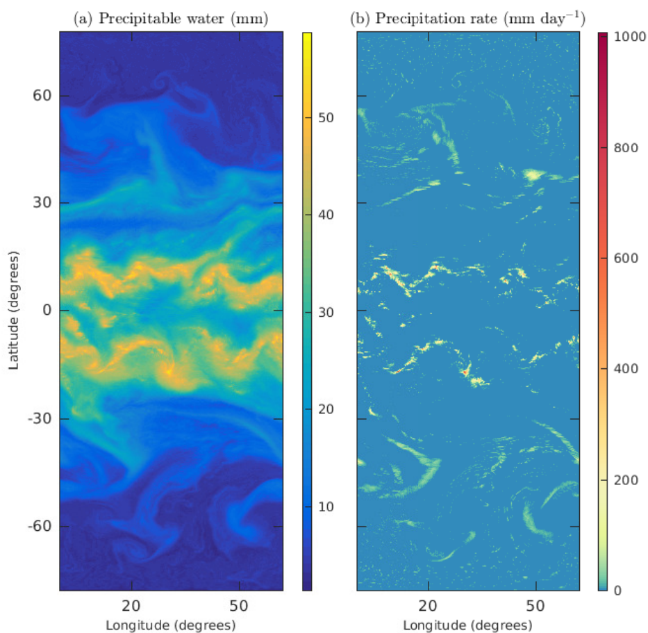
Figure 1. Snapshots of (a) precipitable water (mm) and (b) surface precipitation rate ( \text{mm day}^{-1} ) averaged over a 3-hour period in the control simulation at statistical equilibrium. The model is configured as an equatorial beta plane, and the fields are plotted versus equivalent latitude and longitude. At the largest scales, precipitation is organized by baroclinic eddies in midlatitudes and two ITCZs at low latitudes, but convective organization at a range of length scales is also evident.
