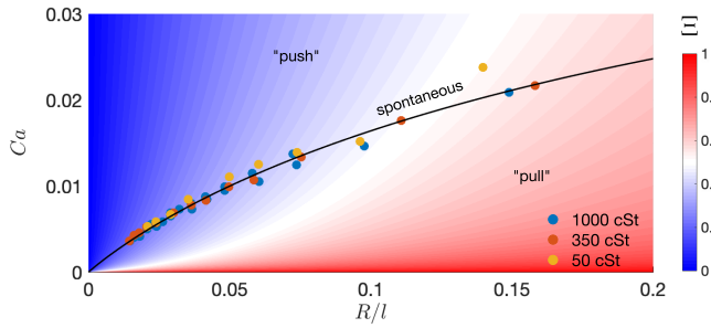
FIG. 3. Phase diagram of forced, rate-controlled imbibition of viscous oil slugs. An external force is needed to move the slug at higher Ca (push) or lower Ca (pull) than the spontaneous rate predicted by Eq. (6) (black solid line). The color of the R/l - Ca space represents the ratios of contact line to total dissipation in such moving slugs, \Xi = \Phi_{cl}/(\Phi_{cl} + \Phi_{bulk}) .
