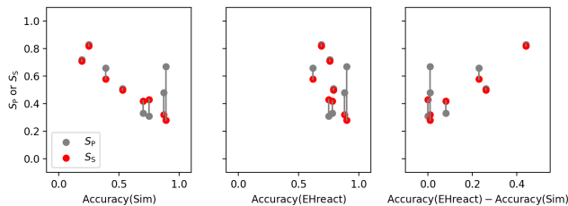
Figure 7. Relationship between the classification accuracy of an assay and the similarity score S_S and the promiscuity score S_P , calculated via similarity (left), EHreact (center) and their difference (right). The lines connect the respective S_S and S_P value of each system. The new EHreact method is much more accurate for non-promiscuous enzymes, or if the new substrate is very similar to substrates in the training set.
