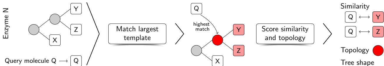
Figure 4. To score the probability of whether a query molecule Q can be processed by enzyme N , the respective template tree is loaded and Q transformed to a list of possible imaginary transitions structures (white squares, only one possibility shown). The ITS of Q is then iteratively matched against the templates (grey circles) in the tree until the most specific (furthest to the right) match is found, highlighted in red. The score then arises from various comparisons of Q to known substrates in the current branch ( Y and Z ), as well as the location of the template within the tree, and the overall shape and diversity of the tree.
