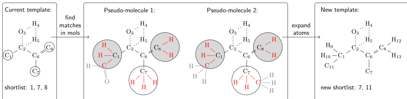
Figure 3. The current template allows atoms 1, 7 and 8 to be extended (not all neighbors specified yet). The neighbors of each shortlisted atom in the template are compared by matching the template to each pseudo-molecule and identifying its neighbors. The algorithm chooses all atoms which have the same neighbors in all pseudo-molecules, here atom 1 and 8 (highlighted in gray), for extending the template, leading to a new, larger, more specific template.
