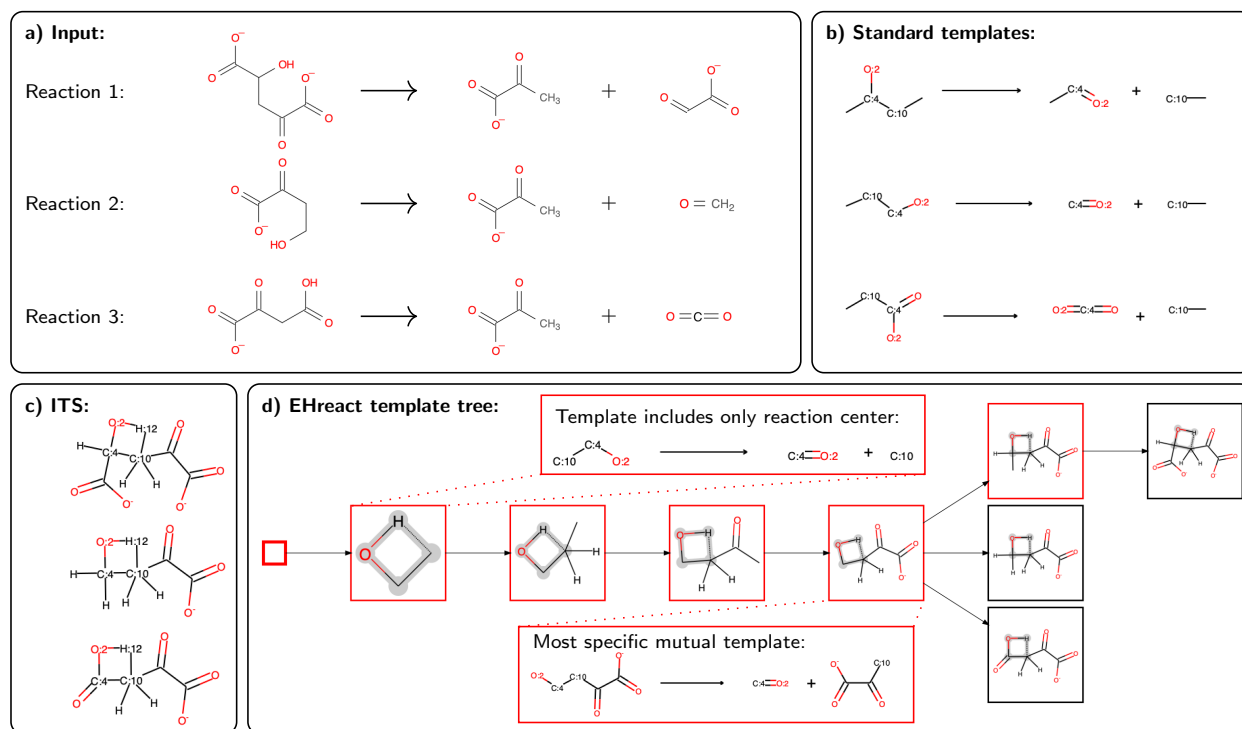
Figure 5. Standard templates and Hasse diagram of three known reactions of 4-hydroxy-2-oxoglutarate lyase (EC 4.1.3.42). Atom-mappings are not shown for atoms not in the reaction center. The inputted reactions (a) are transformed to their respective ITSs (c). An iterative substructure search yields the Hasse diagram of all templates (d), which is reprinted as drawn by EHreact (with the two reaction template drawings added). The reaction center is highlighted in gray. Templates (substructures of the ITS pseudo-molecules) are framed in red, leaf nodes (full ITSs of known reactions) are framed in black. The first template corresponds to the reaction center. The fourth template is the most specific, largest template that describes all inputted reactions, and corresponds to the hand-crafted reaction rule for 4-hydroxy-2-oxoglutarate lyase. In contrast, standard template extraction routines (b), here shown for the common choice of including atoms up to one bond away from the reaction center, lead to three different templates which do not characterize the system well.
