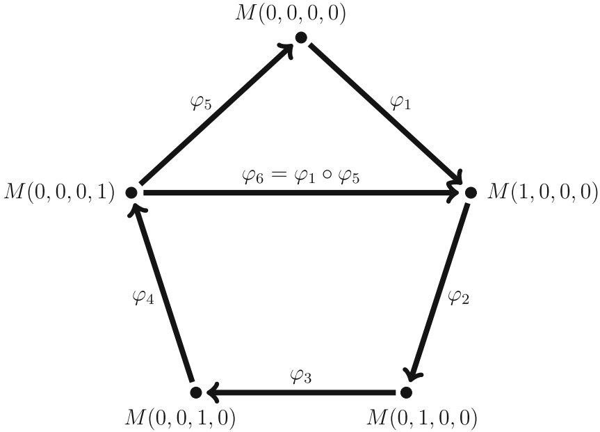
Fig. 1. All non-zero morphisms between finite Verma modules for S_5 . External morphisms have degree 2, and the internal one has degree 4. The morphisms \varphi_1, \dots, \varphi_6 correspond to the singular vectors in R1, ..., R6 in Theorem 3.7
