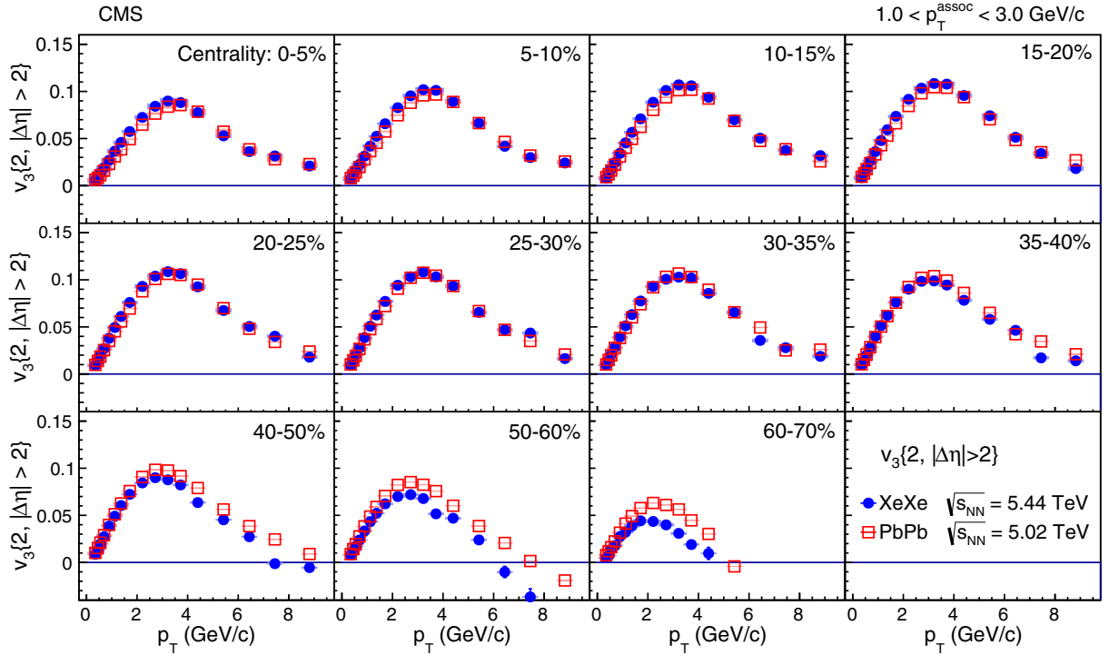
FIG. 7. Comparison of the v_3 results measured with two-particle correlations from two different systems, XeXe collisions at \sqrt{s_{NN}} = 5.44 TeV and PbPb collisions at 5.02 TeV, shown as a function of p_T in 11 centrality bins. The bars (smaller than the marker size) and the shaded boxes represent statistical and systematic uncertainties, respectively.
