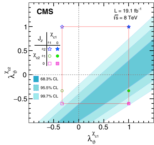
FIG. 3. Two-dimensional \lambda_{\vartheta}^{c2} vs \lambda_{\vartheta}^{c1} contours, at 68.3%, 95.5%, and 99.7% confidence levels (C.L.), measured combining the three J/\psi p_T bins. The physically allowed region (red rectangle) and six pure angular momentum configurations (markers) are also shown. The crossing of the two dashed lines represents the unpolarized case.
