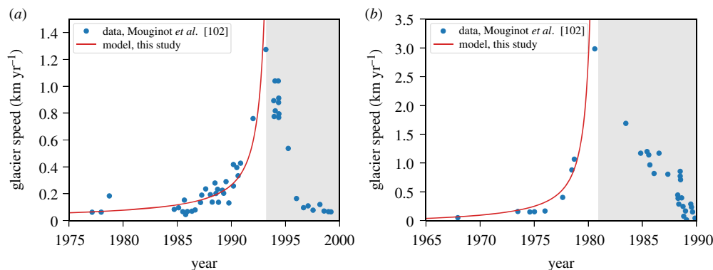
Figure 7. Comparison between our model and observed glacier surface velocities from two surges, (a) L. Bistrup Bræ and (b) Storstømmen , northeast Greenland [102]. Model parameters are the same as in figures 3 and 4, and with b = 0.03 , t_h = 3000 days and initial velocity set according to the data. The greyed regions indicate the slowdown phase of the surge, which our model does not attempt to represent. (Online version in colour.)
