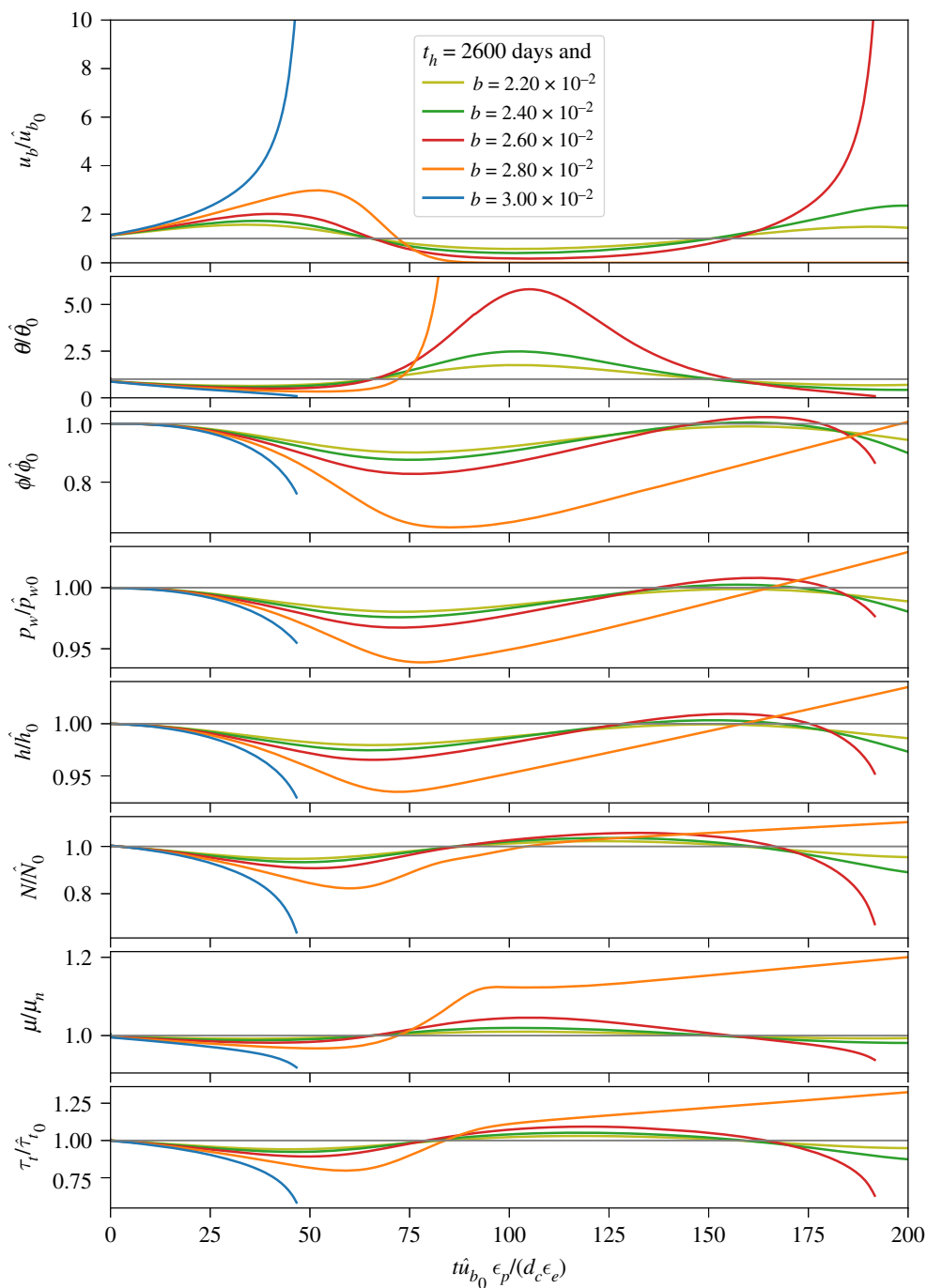
Figure 6. Similar to figure 4 except that models are run using parameter values indicated in figure 5g. Line colours correspond to dot colours in figure 5g. (Online version in colour.)
