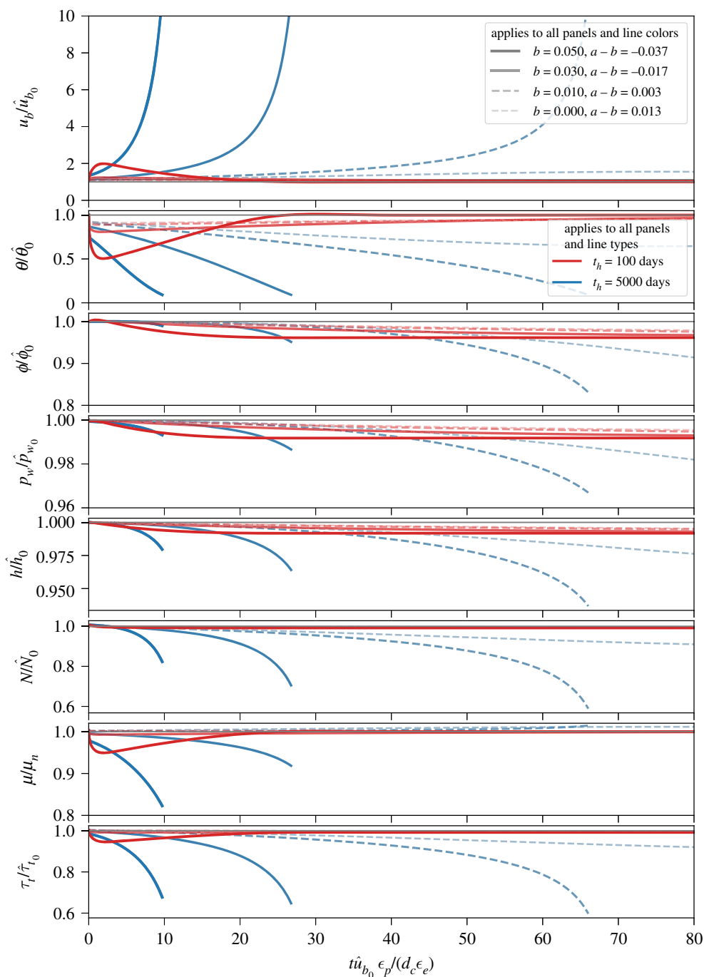
Figure 4. Evolution of (from top to bottom) basal slip rate ( u_b ), state ( \theta ), porosity ( \phi ), pore water pressure in the deforming till layer ( p_w ), ice thickness ( h ), effective pressure ( N ), internal friction coefficient for till ( \mu ) and till shear strength ( \tau_t ) following a perturbation in basal slip rate from steady state for variable ice thickness (S3c). All factors are normalized by their respective initial steady-state values. Velocity perturbation and other parameters are the same as for figure 3. Line thickness and continuity indicate different values of the evolution term b , as indicated in the legend in the upper panel, while line colours indicate values of the hydraulic diffusivity time scale for till ( t_h ), as shown in the legend in the second panel. Dashed lines indicate that the internal friction coefficient is rate strengthening (i.e. (a - b) > 0 ). Truncated lines occur when the integration is stopped; we chose u_b/\hat{u}_{b_0} = 10 , which we define as indicating a surge, as the stopping condition. Over a long enough time scale, the line representing b = 0 and t_h = 5000 days eventually surges. (Online version in colour.)
