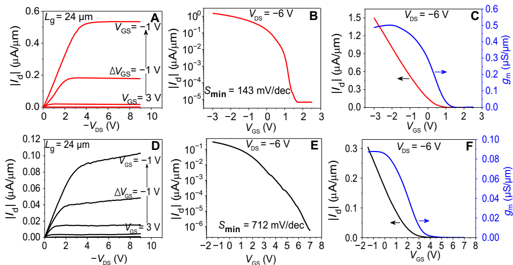
Fig. 4. Comparison of FET characteristics. Comparison of diamond:H/H 2.3 MoO 2.5 (A to C) and diamond:H/MoO 3 (D to F) FET characteristics with the same dimensions: 24- \mu m gate length, 40- \mu m gate width, and 15- \mu m source/drain-to-gate separation: (A versus D) output characteristics, (B versus E) subthreshold characteristics, and (C versus F) transconductance and transfer characteristics (note the different scales).
