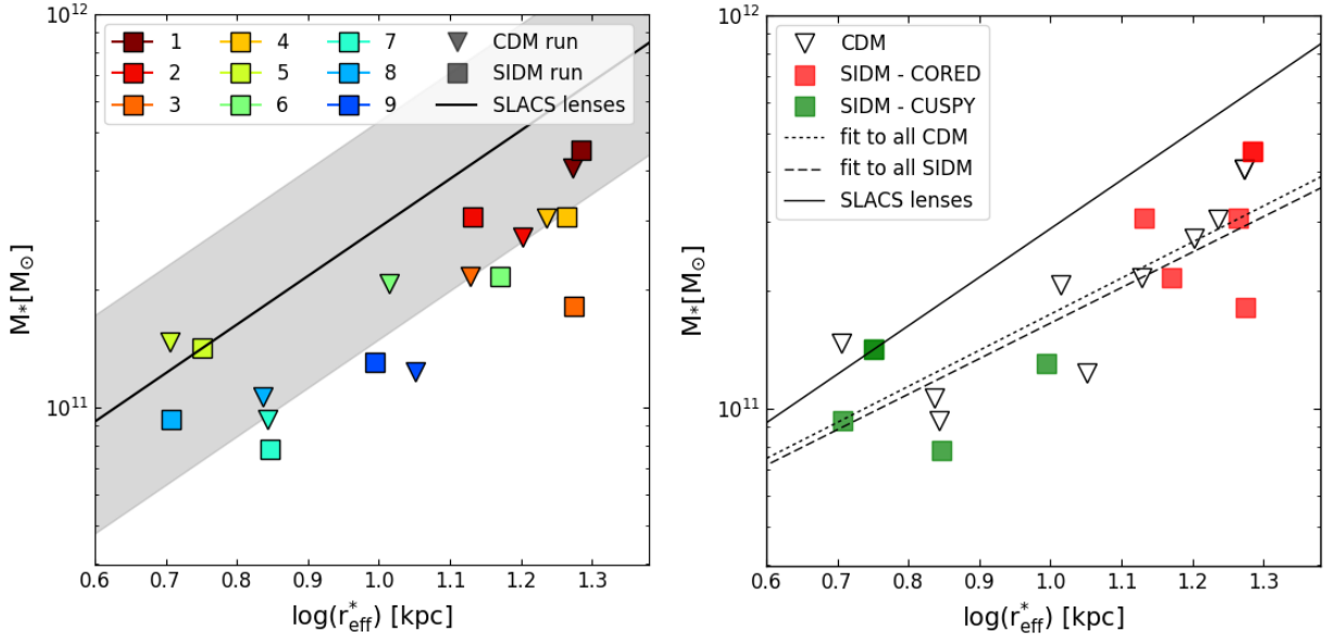
Figure 1. Halo sample in the r_{\text{eff}}^* - M_* plane at z = 0.2 . The black solid line shows the mean relation derived for the SLACS lenses by Auger et al. (2010b), together with the scatter of the data (gray band) calculated from the intrinsic scatter of the data and the uncertainty on the linear fit. Left panel: the coloured squares and triangles show how the halo properties change between the CDM and SIDM run. Right panel: we show the same points as in the left panel, but here the systems are color-coded according to the final profile properties; the dotted and dashed black lines show the best-fit linear relation to the full sample of, respectively, CDM and SIDM haloes.
