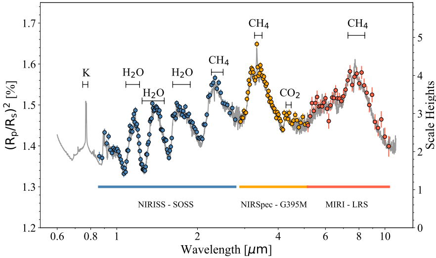
Fig. 11. Synthetic transmission spectrum model of TOI-674b (gray line) in the JWST spectral range computed with petitRADTRANS (Mollière et al. 2019). The model assumes solar abundance and a cloud-free atmosphere with an isothermal temperature of 700 K. PandExo (Batalha et al. 2017) simulations of TOI-674b transmission spectrum observations made with JWST instruments NIRISS (blue), NIRSpec (orange), and MIRI (red) are also shown.
