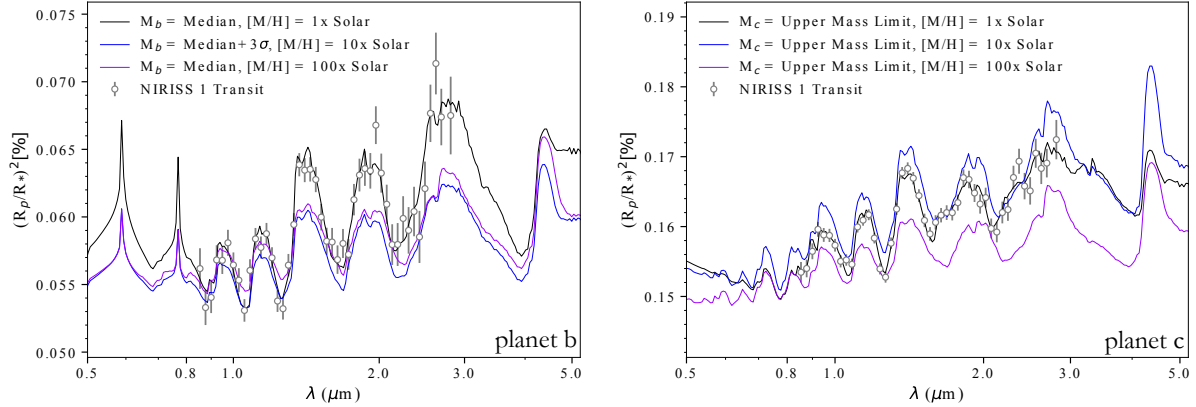
Figure 10. Models generated for planets b and c in the left and right panels, respectively. Each panel shows three models describing plausible atmospheric scenarios. In black we present an atmospheric model which has a metallicity of 1\times solar, considering the RV extracted median mass and upper mass limit for planets b and c, respectively. In purple we present an atmospheric model which has a metallicity of 100\times solar considering the RV extracted median mass and upper mass limit for planets b and c, respectively. In blue we present an atmospheric model which has a metallicity of 10\times solar, however we consider the RV extracted median mass plus the 3\sigma upper uncertainty for planet b and the upper mass limit for planet c. We overplot the simulated JWST NIRISS/SOSS observations for the 1\times solar case to emphasise the precision we would obtain from a single transit observation.
