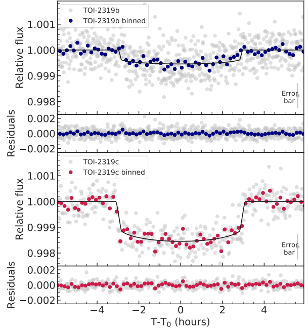
Figure 7. Phase-folded TESS light curve of HD 152843 b (upper panel) and HD 152843 c (lower panel). Nominal TESS data are shown in light gray together with 10-min binned data in solid colour. The inferred transit model for each planet is over-plotted with a solid black line. An example of the nominal white noise in the data is also shown.
