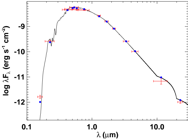
Figure 5. Spectral energy distribution of HD 152843. Red symbols represent the observed photometric measurements, where the horizontal bars represent the effective width of the passband. Blue symbols are the model fluxes from the best-fit Kurucz atmosphere model (black).
