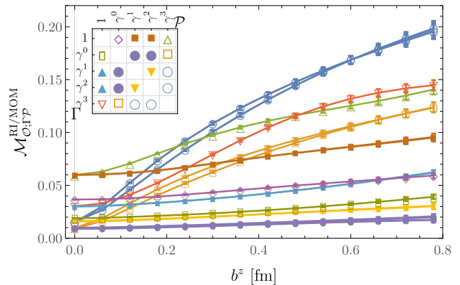
FIG. 3. Submatrix of the RI'/MOM mixing matrix \mathcal{M}_{O_{TP}}^{\text{RI'/MOM}}(p_R) [Eq. (26)] for quark bilinear operators with straight Wilson lines ( b_T = 0 ) with various extents b^z , for momentum n^\nu = (2, 2, 2, 2) in lattice units, calculated on the E_{32} ensemble.
