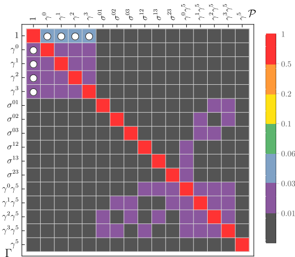
FIG. 2. RI'/MOM mixing pattern \mathcal{M}_{O_{TP}}^{\text{RI'/MOM}} [Eq. (26)] for local quark bilinear operators, calculated on the E_{32} ensemble. White circles indicate the pattern of mixings predicted based on the off-shell nature of the quark in the relevant Green's functions [60].
