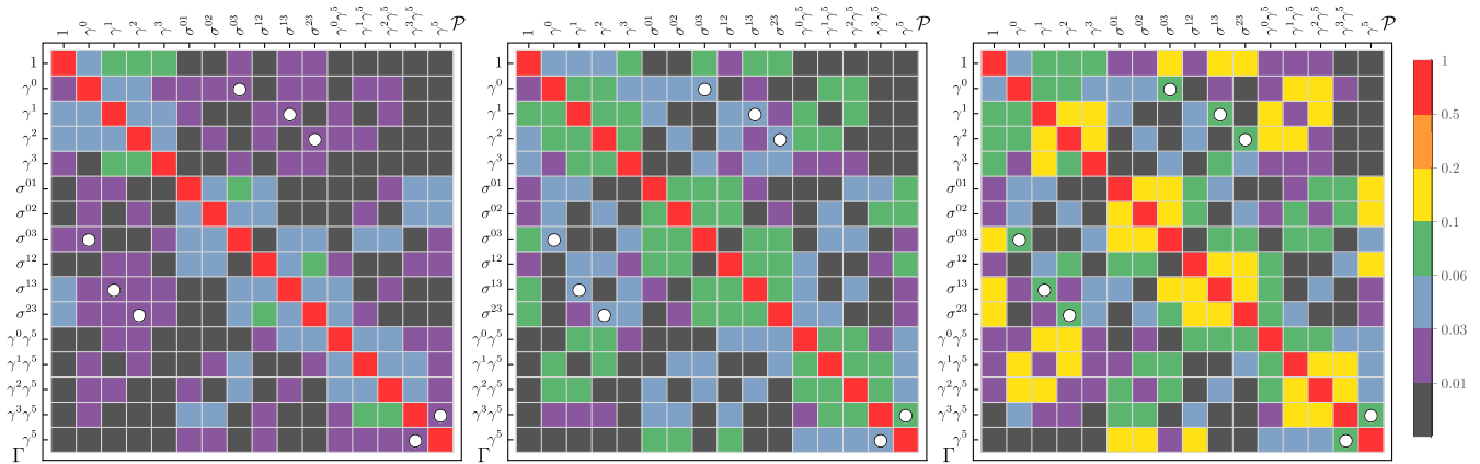
FIG. 6. RI'/MOM mixing pattern \mathcal{M}_{\mathcal{O}_{TP}}^{\text{RI'/MOM}} [Eq. (26)] for quark bilinear operators with symmetric ( b_T = 0 ) staple-shaped Wilson lines. From left to right, panels show results for operators with b_T/a = \{3, 7, 11\} and \eta/a = 14 , calculated on the E_{32} ensemble. White circles indicate the mixings predicted by one-loop lattice perturbation theory [56].
