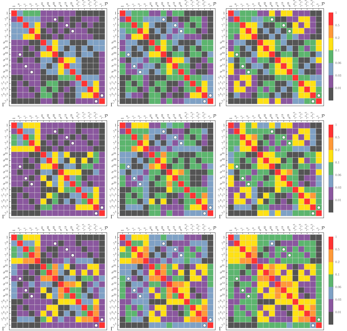
FIG. 7. RI'/MOM mixing pattern \mathcal{M}_{\mathcal{O}_{\Gamma P}}^{\text{RI'/MOM}} [Eq. (26)] for quark bilinear operators with asymmetric staple-shaped Wilson lines ( b^z, b_T \neq 0 ) and \eta/a = 14 , calculated on the E_{32} ensemble. From left to right, panels show results for operators with b_T/a = \{3, 7, 11\} , and from top to bottom with b^z/a = \{3, 7, 11\} . For the asymmetric staple, there are no predictions available for the mixing patterns from one-loop lattice perturbation theory.
