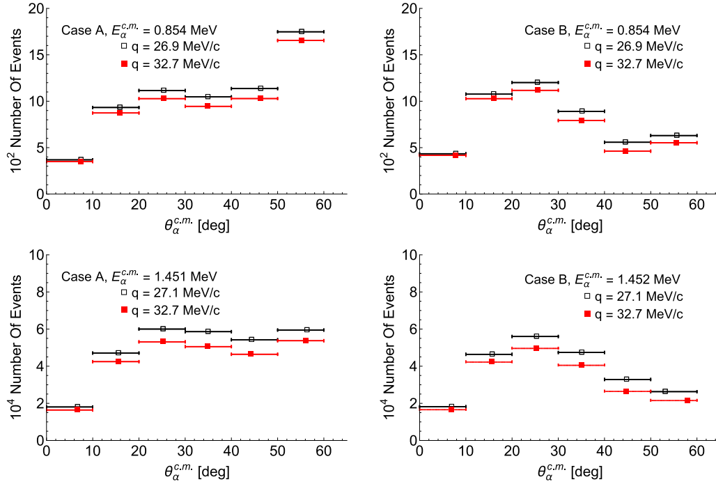
FIG. 21. Number of events as a function of \theta_{\alpha}^{c.m.} assuming 100 days of data collection at the luminosity of 2.5 \times 10^{36} \text{ cm}^{-2} \text{ s}^{-1} . The left column represents t_{C0} case A and the right one case B. Horizontal bars denote the width of the \theta_{\alpha}^{c.m.} bin, which here is equal to 10^\circ . Horizontal placement of the data point within a bin was done according to the procedure recommended in Ref. [64]. The q bins are 1.91 MeV/c wide and E_{\alpha}^{c.m.} bins are 100 keV. For all events inside a particular q and E_{\alpha}^{c.m.} bin, the specified q values represent the average value, and the stated E_{\alpha}^{c.m.} values represent the average of the expected and averaged E_{\alpha}^{c.m.} value.
