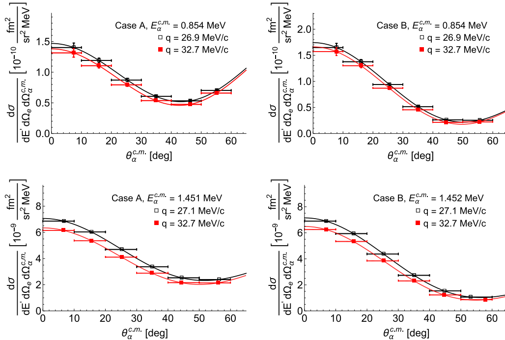
FIG. 22. Differential cross section as function of \theta_{\alpha}^{c.m.} . The left column represents t_{C0} case A and right column is case B. Vertical bars correspond to statistical uncertainties assuming 100 days of data collection at the luminosity of 2.5 \times 10^{36} \text{ cm}^{-2} \text{ s}^{-1} . The same binning procedure was performed as described in caption of Fig. 21.
