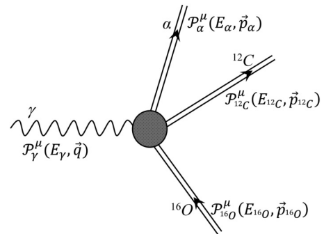
FIG. 2. Feynman diagram for the photodisintegration of ^{16}\text{O} involving a real photon, \gamma , which requires that q = \omega = E_\gamma . The kinematic variables here will be discussed in more detail in Sec. III.
