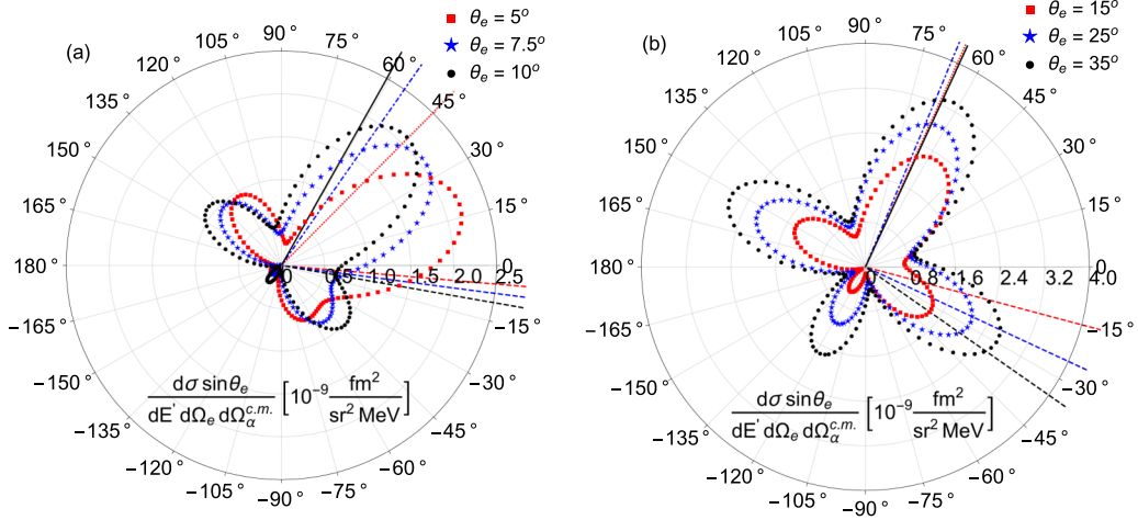
FIG. 11. Angular distribution of the ^{16}\text{O}(e, e'\alpha)^{12}\text{C} differential cross section multiplied by \sin\theta_e for beam energy of E_e = 114 MeV, E_\alpha^{\text{c.m.}} = 1.5 MeV, for different electron scattering angles \theta_e = 5^\circ, 7.5^\circ, 10^\circ (a); 15^\circ, 25^\circ, 35^\circ (b). The electron beam lies on a ray from 180^\circ to 0^\circ , the directions of the scattered electrons are represented by dashed lines, and the other type of lines on the positive angle side represents the direction of the virtual photon in the laboratory system.
