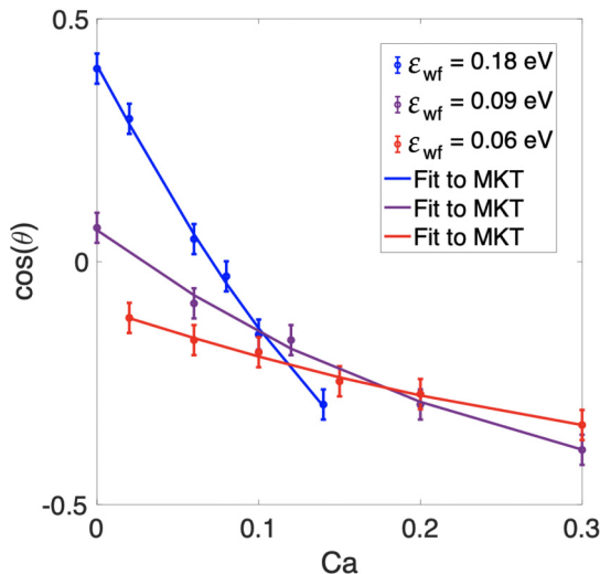
FIG. 4. Dynamic contact angles as a function of Ca , for various wall-fluid interactions for H = 40 \text{ \AA} . Solid lines denote fits to MD data (symbols) using Eq. (4).
