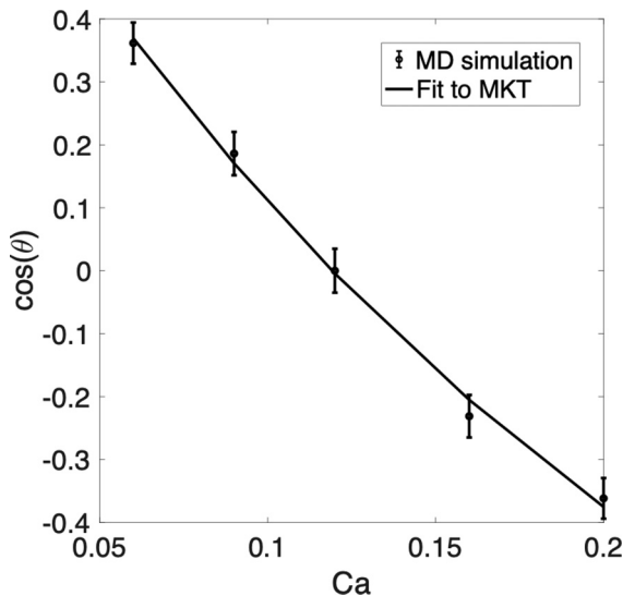
FIG. 5. Dynamic contact angles as a function of Ca , for \varepsilon_{wf} = 0.18 eV, \beta_{ij}^p = 0.21 , and H = 30 Å. The solid line denotes a fit to MD data (symbols) using Eq. (4).
