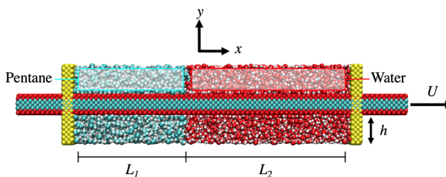
FIG. 1. MD System Setup: The solid wall serves to bound the fluids in a slit geometry; it also imposes a translation speed of U in the positive x direction. The wall consists of two different groups of wall particles (interactions are identical), shown in cyan and red. The former (inner) group is not thermostatted and is used to impose the translation of the whole structure; the latter (outer) group, is thermostatted using a Langevin thermostat. Fixed walls that constrain the fluid in the axial direction are shown in yellow. Periodic boundary conditions are imposed in all dimensions.
