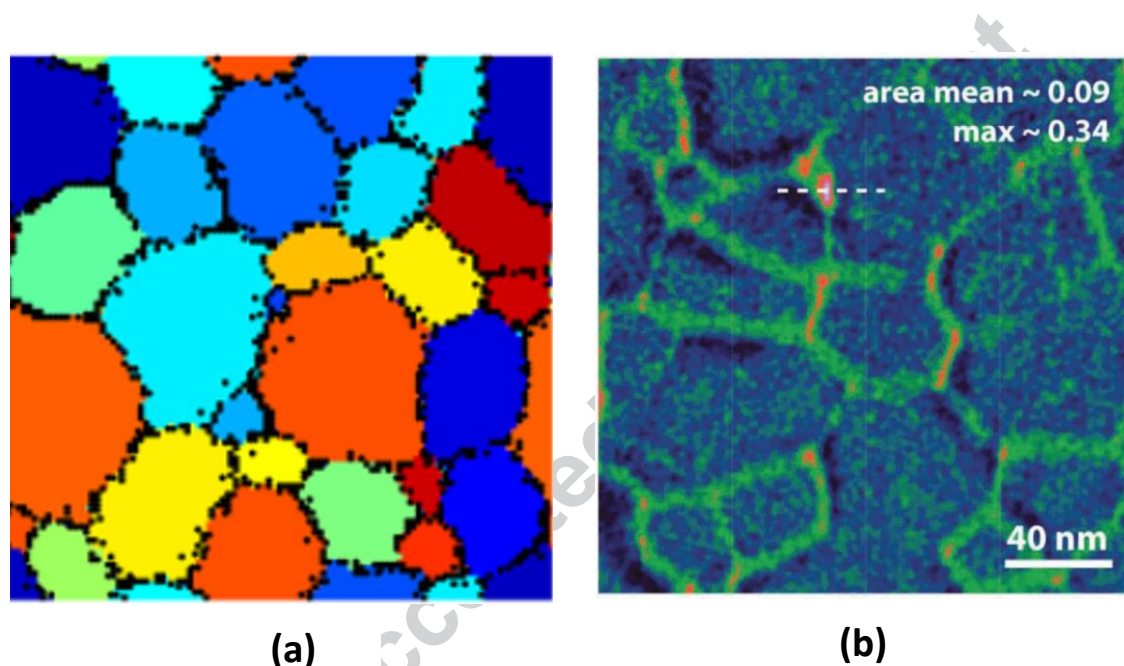
Figure 1. Nanocrystalline alloys can be stabilized by segregation of solutes to the boundaries, lowering the boundary energy and also providing kinetic impediments to grain-boundary migration. This is illustrated by equilibrium Monte Carlo simulations for a body-centered-cubic (bcc) alloy structure,[58] and by scanning transmission electron microscopy and chemical mapping by energy dispersive spectroscopy of a Au-Pt alloy.[59] The simulated structure in (a) is for a generic bcc material and has no formal length scale, although the edge length spans 100 atoms, which for bcc tungsten amounts to ~30 nm.
