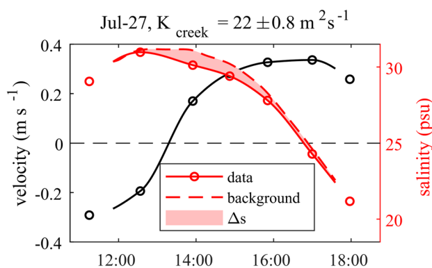
Fig. 13 Time-series of velocity (black line), salinity (red lines), and salinity anomaly (red shading) at transect 5. The dispersion rate due to trapping in the creeks is calculated from the tidal correlation between the salinity anomaly and the tidal velocity
