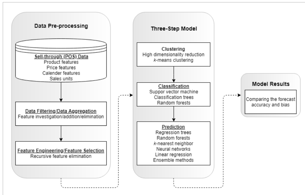
Fig. 1: The proposed methodology
