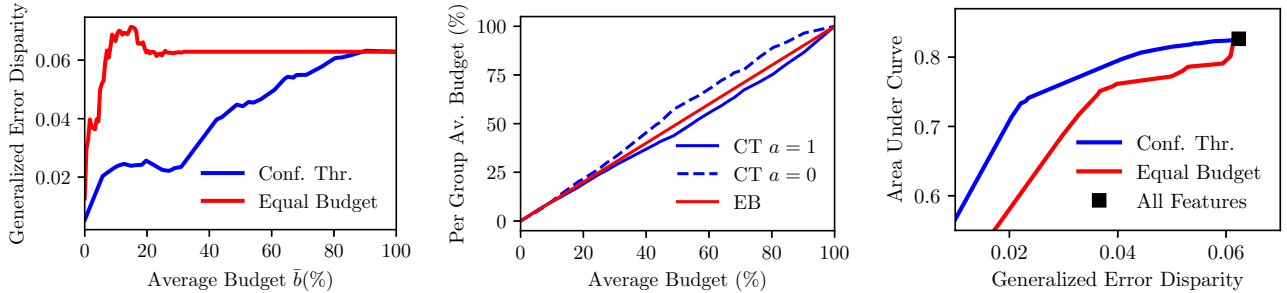
Figure 2: Confidence thresholds for achieving equal generalized error rates across the Urban and Rural subgroups in the Mexican Poverty dataset. In each plot, the curves are generated by sweeping the target error rate \beta_{err} , changing the average budget allocated to each groups. Left, the residual error disparity for the confidence thresholds (blue) and the equal budget benchmark (red). Center, the average average budget per group versus the total average budget. The dashed and solid blue lines represent the average budget used for respectively the Urban ( a = 1 ) and Rural ( a = 0 ) subgroups while the red line represents the average budget for both groups using the benchmark method. Right: The Pareto front of the AUC versus disparity trade-off for our method and the benchmark method as well as for the classifier with access to all features in black.
