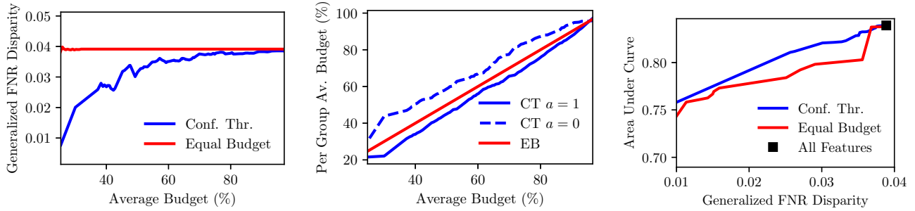
Figure SM2: Confidence thresholds for achieving equal generalized FNR rates across the Urban and Rural subgroups in the Mexican Poverty dataset. In each plot, the curves are generated by sweeping the target error rate \beta_{fnr} . Left: the residual generalized FNR disparity for the confidence thresholds (blue) and the equal budget benchmark (red). Center: The average budget per group versus the total average budget across groups. The dashed and solid blue lines represent the average budget used for respectively the Urban ( a = 1 ) and Rural ( a = 0 ) subgroups while the red line represents the average budget for both groups when using the benchmark method. Right: The Pareto front of the AUC-disparity trade-off for our method and the benchmark method. The black square represents the classifier that has access to all features.
