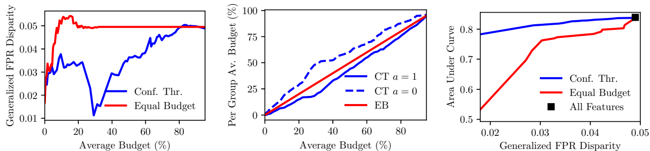
Figure 3: Confidence thresholds for achieving equal generalized FPR rates across the Urban and Rural subgroups in the Mexican Poverty dataset. In each plot, the curves are generated by sweeping the target error rate \beta_{fpr} . Left, the residual generalized FPR disparity for the confidence thresholds (blue) and the equal budget benchmark (red). Center, the average budget per group versus the total average budget. The dashed and solid blue lines represent the average budget used for respectively the Urban ( a = 1 ) and Rural ( a = 0 ) subgroups while the red line represents the average budget for both groups when using the benchmark method. Right, the Pareto front of the AUC-disparity trade-off for our method and the benchmark method. The black square represents the classifier that has access to all features.
