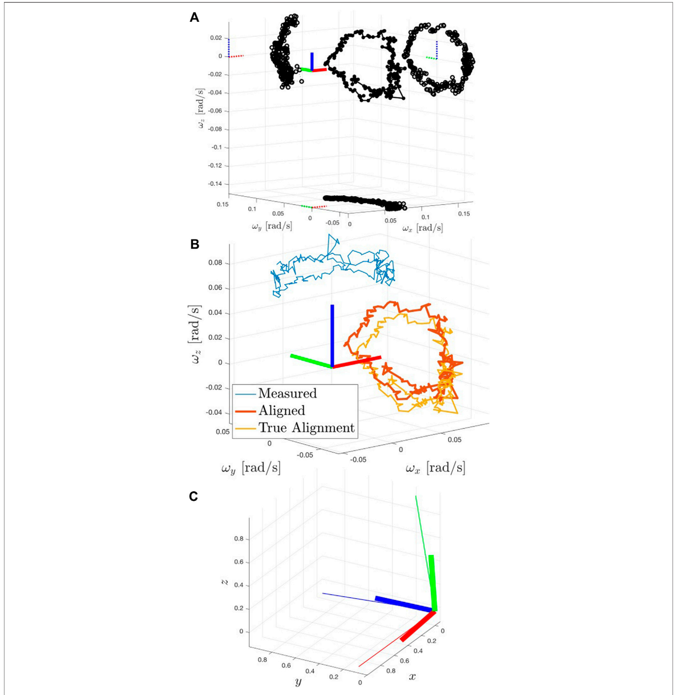
FIGURE 8 | (A) Resulting polhode after alignment to the Target’s estimated principal axes. The polhode’s plane projections produce central conics (not rotated nor displaced from their respective origins). Solid circles indicate the polhode, and open circles indicate the projected conics. (B) Polhode comparison between the measured (blue, in geometric frame), aligned (red, after rotating by the estimated orientation from geometric to principal axes), and groundtruth-aligned (orange) curves. (C) Visual comparison of the offset between the groundtruth principal axes (bold RGB triad) against the estimated orientation (thin, longer RGB triad).
