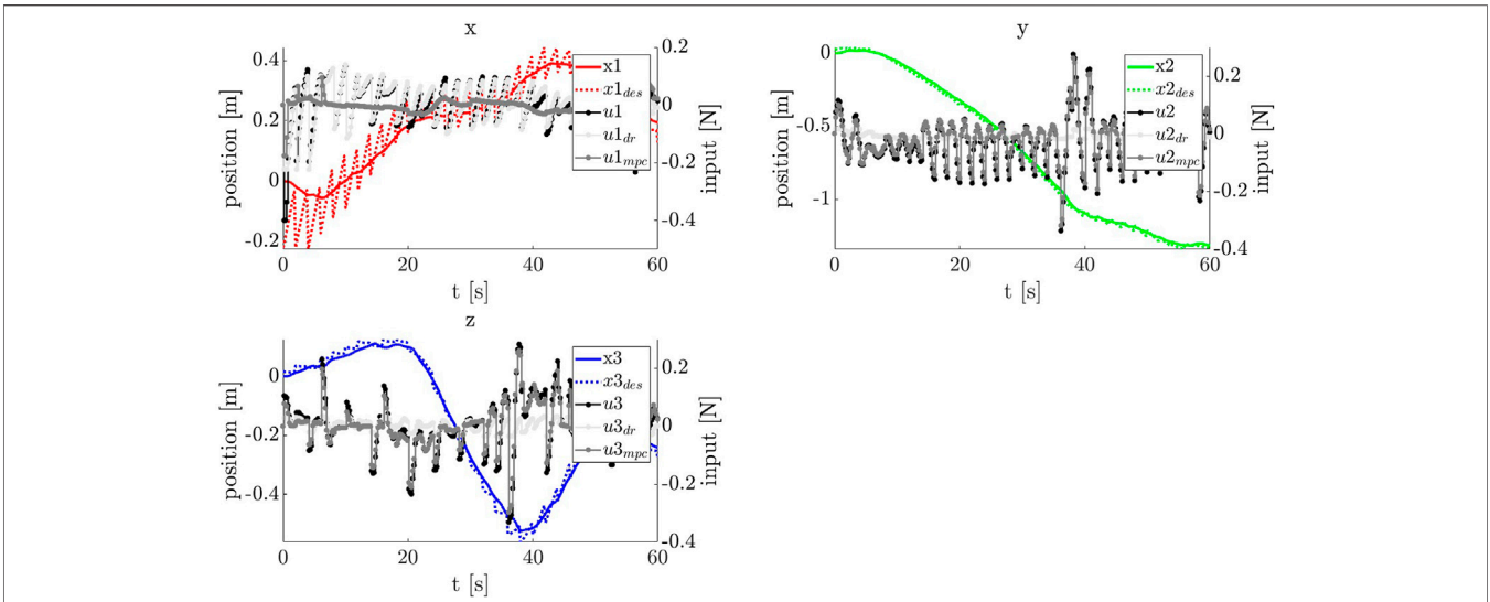
FIGURE 13 | The input and state histories for the robust controller tracking the online-updated reference trajectory (dashed). It is important to remember that the reference trajectory in this scheme actually shifts in real-time as new SLAM estimates of the true Target attitude, \hat{q}_T become available. It is precisely this stepwise shifting for which the tube robustness guarantee is produced. u_{dr} indicates the disturbance rejection component, while u_{mpc} indicates the nominal MPC component.
