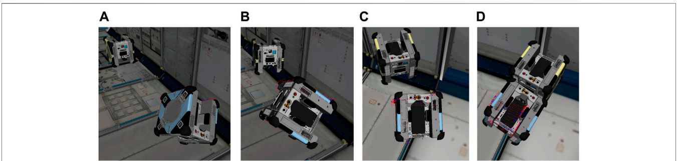
FIGURE 14 | A timelapse of the rendezvous portion of the pipeline for an arbitrary tri-axial tumble. (A–D) , the Chaser begins tracking the motion plan with its robust controller while periodically updating the inertial frame reference trajectory based on SLAM estimates of \hat{q}_T .
