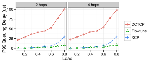
Figure 13: Flowtune keeps 2-hop and 4-hop 99 th -percentile queuing delays below 8.9 \mu s. At 0.8 load, XCP has 3.5 \times longer queues, DCTCP 12 \times . pFabric and sfqCoDel do not maintain FIFO ordering so their p99 queuing delay could not be inferred from sampled queue lengths.
