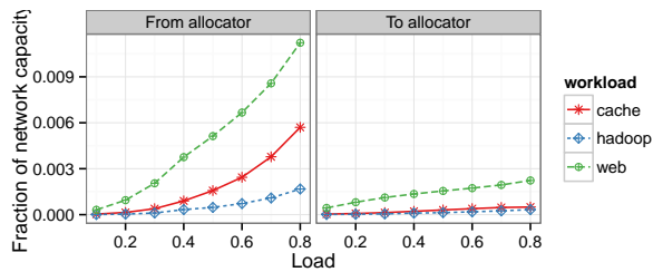
Figure 9: Overhead with Hadoop, cache, and Web workloads is < 0.17\% , 0.57\% , and 1.13\% of network capacity.
