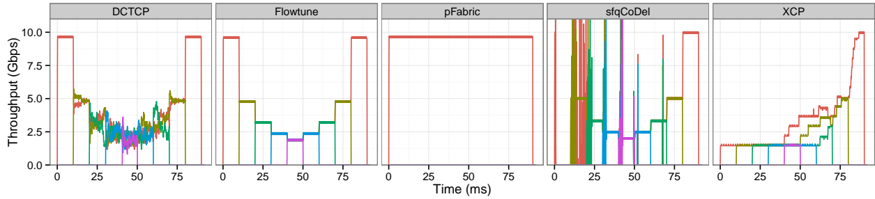
Figure 8: Flowtune achieves a fair allocation within 100 \mu s of a new flow arriving or leaving. In the benchmark, every 10 ms a new flow is added up to 5 flows, then flows finish one by one. DCTCP approaches a fair allocation after several milliseconds. pFabric, as designed, doesn't share the network among flows. sfqCoDel gets a fair allocation quickly, but retransmissions cause the application to observe bursty rates. XCP is conservative in handing out bandwidth and so converges slowly.
