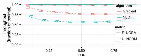
Figure 17: Normalizing with F-NORM achieves close to optimal throughput, while avoiding over-capacity allocations. U-NORM’s throughput is low in comparison.
