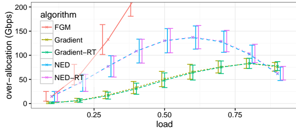
Figure 16: Normalization is necessary; without it, optimization algorithms allocate more than link capacities.
