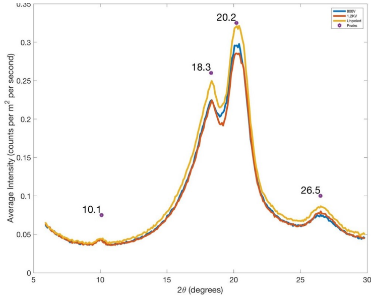
Figure 3. X-ray diffraction image of unpoled commercial PVDF fiber. The peak at 2\theta = 20.26^\circ is related to the diffraction of \beta phase at (110) and (200) crystal planes. The peaks at 18.3^\circ and 26.5^\circ are indicative of alpha phase at (020) and (021) crystal plane, respectively.
