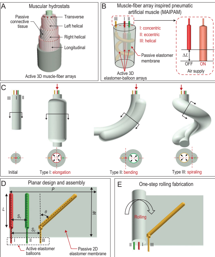
Figure 1. Design and fabrication principle of the MAIPAMs. (A) Schematic of the skeleton-free muscular hydrostats. Muscular hydrostats mainly consist of active three-dimensional (3D) muscle-fiber arrays (including transverse, left-helical, right-helical and longitudinal muscle fibers) reinforced by passive connective tissues, enabling multiple-mode actuations and versatile manipulation by selectively actuating the muscle-fiber arrays. (B) The morphology of the designed MAIPAMs, consisting of active 3D elastomer-balloon arrays (cylinder latex elastomer balloon with an outer diameter of 5 mm and a wall thickness of 0.3 mm) reinforced by a passive 2D elastomer membrane (3M VHB 4910 with inherent strong adhesive, a thickness of 1 mm). The arrays contain three kinds of active elastomer balloons: concentric (type I), eccentric (type II) and helical (type III) active elastomer balloons. (C) Multiple-mode actuations of the MAIPAMs. Upon a supplied pressure, the elongation of active elastomer balloons can be converted into elongation (type I balloon), bending (type II balloon) and spiraling (type III balloon), respectively. (D) Schematic of the planar design and assembly of the MAIPAMs (Fig. S2 and Movie S1): (i) determine the design parameters of active elastomer balloons (including the length L of the active elastomer balloon, the distance S between the active elastomer balloon and the edge of the passive elastomer membrane, and the oblique angle \theta ); (ii) assemble the active elastomer balloons in a passive 2D elastomer membrane. (E) Working principle of the one-step fabrication approach for rolling the passive 2D elastomer membrane into a 3D MAIPAM (Movie S1).
