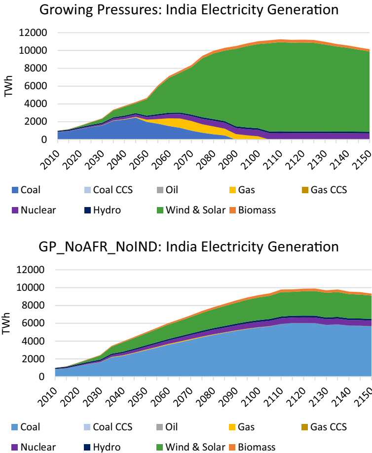
Fig. 17 Electricity generation mix in India in the Growing Pressures scenario and the GP_NoAFR_NoIND scenario in which India and Africa take limited action to reduce fossil fuels
