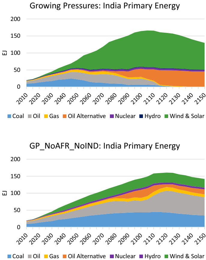
Fig. 16 Primary energy mix in India in the Growing Pressures scenario and the GP_NoAFR_NoIND scenario in which India and Africa take limited action to reduce fossil fuels
