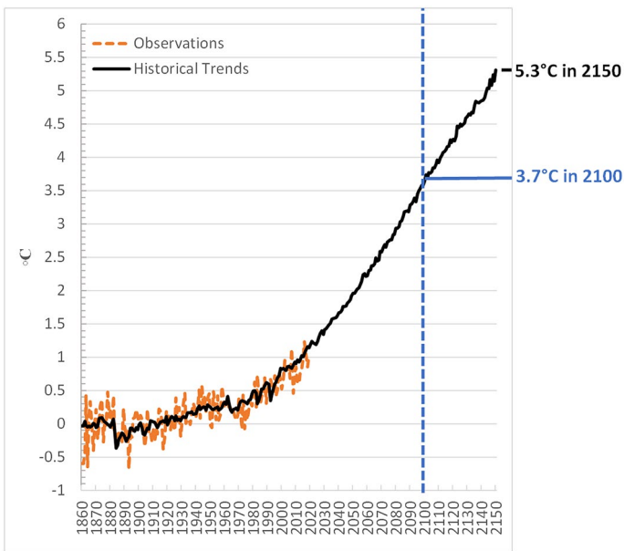
Fig. 5 Global annual mean surface air temperature relative to pre-industrial levels (1861–1880 mean) under the Historical Trends scenario
