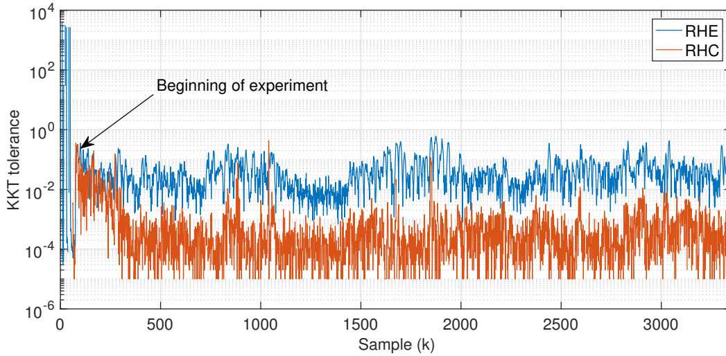
Figure 13: KKT tolerances
