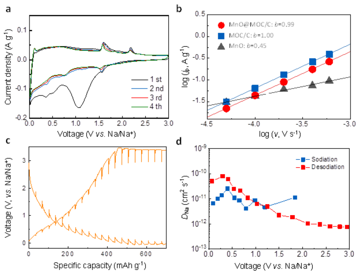
Figure 5. Electrochemical mechanism of MnO@MOC/C hybrid in SIBs. (a) CV curves at 0.1 mV s -1 (b) b -values analysis and (c) GITT of MnO@MOC/C. (d) Na + diffusion coefficient ( D Na ) calculated from GITT.
