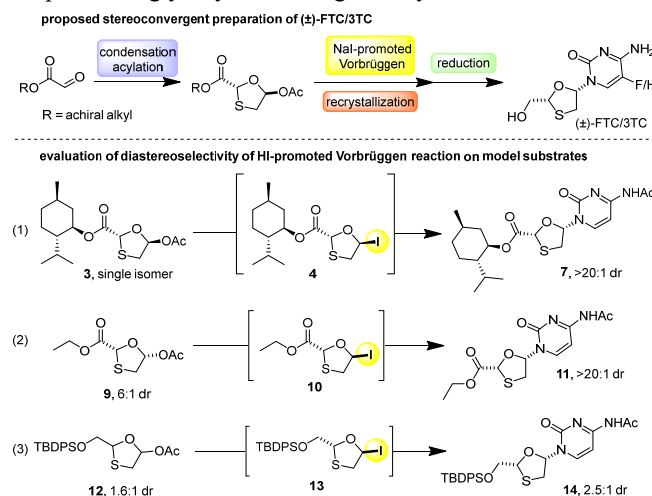
Figure 4. (top) Proposed route to (±)-FTC/3TC. (bottom) Mechanistic investigation of HI-promoted Vorbrüggen glycosylation using I 2 -triethylsilane.
