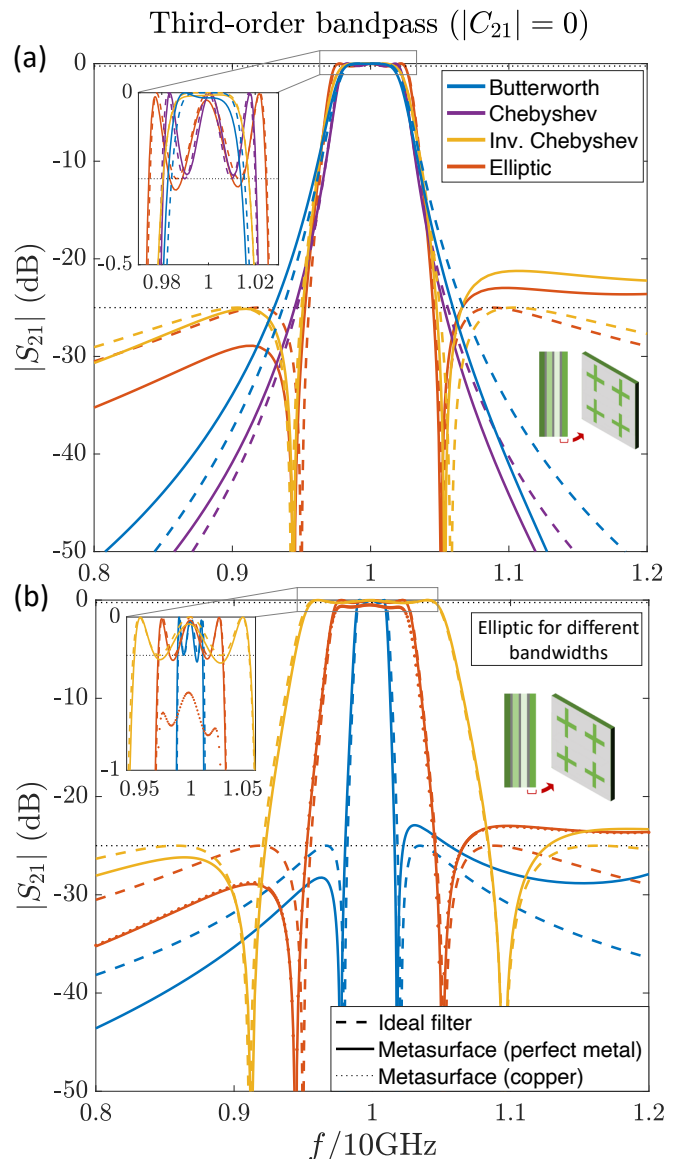
FIG. 4. Optimized third-order bandpass filters (a) of different types with same bandwidth and (b) elliptic only for different bandwidths. We use the same structure as in Fig. 3 but with three metallic sheets and four dielectric layers. Physical parameters and 3dB bandwidths are provided in Table I. We notice good agreement of lossless structures (solid lines) with ideal filters (dashed lines), except for small deviations mainly due to effects from high-order modes. Copper losses (dotted line) reduce peak transmission while preserving the filter's shape.
