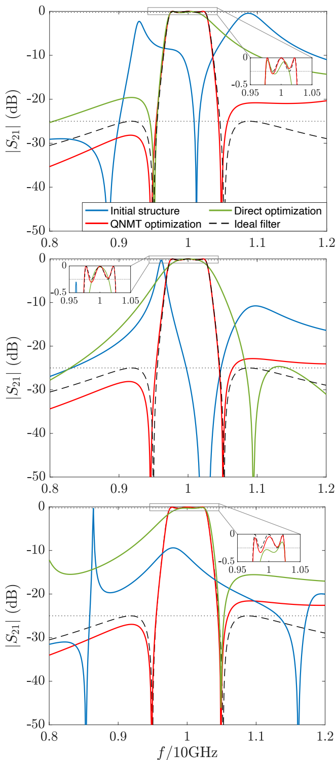
FIG. 8. Different optimization solutions for a desired third-order bandpass elliptic SF (black dashed lines). Starting with three different initial structures (blue lines), the solutions obtained with our QNMT method (red lines; structural parameters in Table I) match the SF, while local optima obtained by directly optimizing the transmission spectrum at few key frequencies (green lines) fail.
