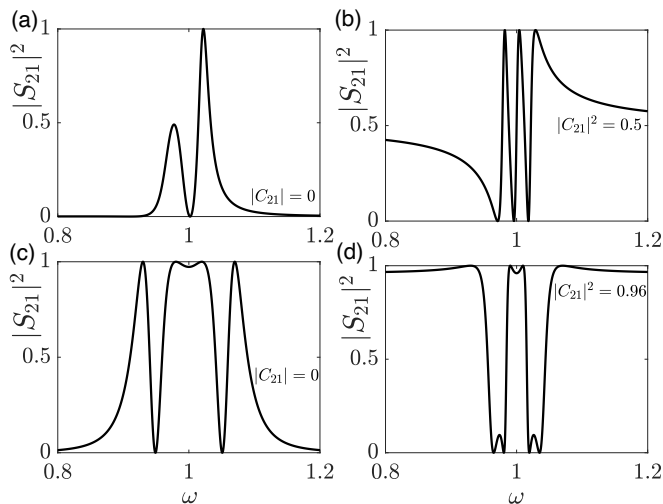
FIG. 9. Non-standard S_{21} spectra of symmetric two-ports with C = \begin{pmatrix} ir & t \\ t & ir \end{pmatrix} and resonances: (a) \omega_n = (0.968 - 0.02i, 0.99 - 0.02i, 1.02 - 0.01i) , \sigma_n = (1, -1, -1) , t = 0 , (b) \omega_n = (0.98, 1, 1.02) - 0.005i , \sigma_n = (1, 1, 1) , t^2 = 0.5 , (c) \omega_n = (0.94, 0.95, 1.05, 1.06) - 0.02i , \sigma_n = (1, 1, -1, -1) , t = 0 , (d) \omega_n = (0.96 - 0.01i, 0.984 - 0.004i, 1.016 - 0.004i, 1.04 - 0.01i) , \sigma_n = (-1, 1, -1, 1) , t^2 = 0.96 .
