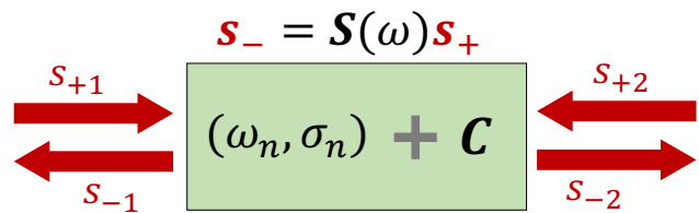
FIG. 1. A lossless reciprocal two-port scattering system excited at frequency \omega , with input and output amplitudes respectively s_{\pm p} , related by the S -matrix through s_- = S s_+ . The system supports high- Q quasi-normal modes (QNMs) with frequencies \omega_n and port-coupling ratios \sigma_n , while low- Q resonances create an effective background response C .
