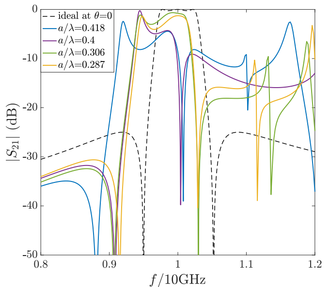
FIG. 10. TM-to-TM transmission at angle \theta = 15^\circ for the different optimized structures in Figs. 4, 8 with ( \sim 6\% bandwidth) elliptic response at normal incidence. The angle response deviates more as the period increases.
