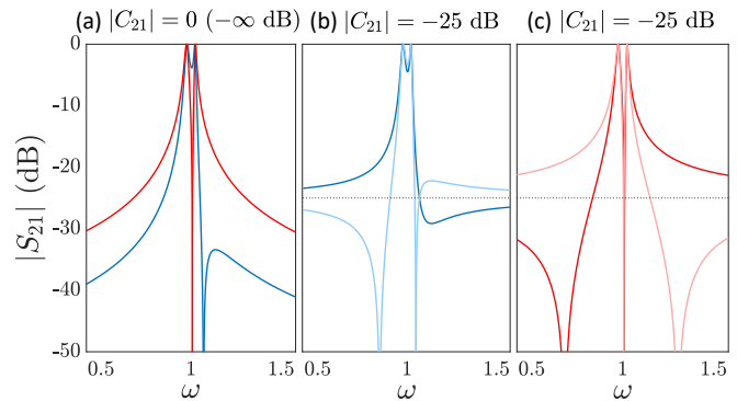
FIG. 2. Second-order filter responses, using QNM expansions of the form S = \bar{S}C , with two modes of frequencies \omega_n = (0.98 - 0.01i, 1.02 - 0.005i) and coupling ratios (\pm\sigma, \pm\sigma) in \bar{S} , and with unitary reciprocal C = \begin{pmatrix} i\sigma^* r & t \\ t & i\sigma r \end{pmatrix} where r = \sqrt{1 - t^2} and such that i\sigma\beta = -1 and C_{22} = \sigma^2 C_{11} ( \Leftrightarrow S_{22} = \sigma^2 S_{11} ), for different values of real background transmission t indicated in the plots. We use the RWA of ignoring negative-frequency poles, so the amplitudes of S -matrix coefficients are exactly the same for any complex \sigma = \sqrt{\gamma} = e^{i\varphi/2} . A zero always occurs between modes of same coupling ratio (red), so filters with no zeros between the poles require opposite signs of the ratios (blue). Including negative-frequency poles would result to the same qualitative behavior and only slightly change the response away from the resonances.
