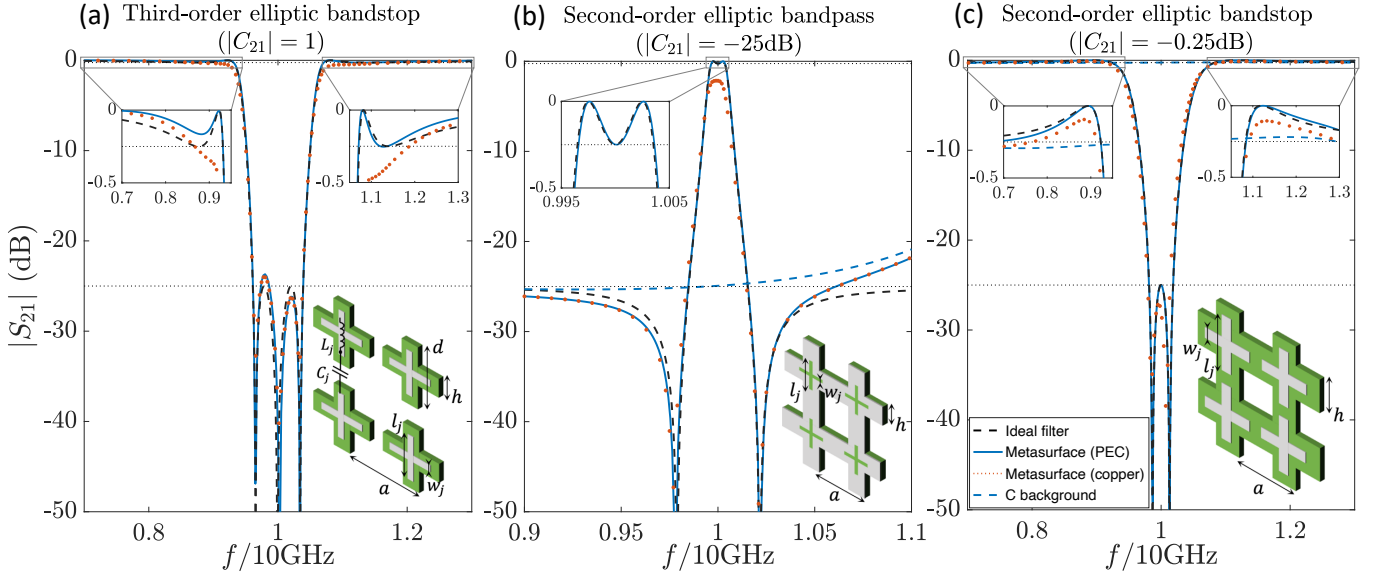
FIG. 5. (a) Third-order elliptic bandstop filter. The structure has three metallic-cross arrays and four dielectric layers with parameters: a = 17.05\text{mm} , h/a = 0.03 , d/a = 0.619 , w/a = (1.53, 3.73, 1.61) \times 10^{-3} , l/a = (0.558, 0.589, 0.524) , t/a = (0.166, 0.358, 0.441, 0.183) , \epsilon = (4.76, 3.22, 4.05, 4.50) . (b) Second-order elliptic bandpass filter. The symmetric structure has two metallic sheets and three dielectric layers with parameters: a = 17.571\text{mm} , h/a = 0.456 , w_{1,2}/a = 6.08 \times 10^{-3} , l_{1,2}/a = 0.4355 , t_{1,3}/a = 0.3072 , t_2/a = 0.3169 , \epsilon_{1,3} = 3.82 , \epsilon_2 = 1.893 . (c) Second-order elliptic bandstop filter. The symmetric structure has two metallic-cross arrays and three dielectric layers with parameters: a = 18.66\text{mm} , h/a = 0.181 , w_{1,2}/a = 2.74 \times 10^{-3} , l_{1,2}/a = 0.514 , t_{1,3}/a = 0.204 , t_2/a = 0.332 , \epsilon_{1,3} = 1.60 , \epsilon_2 = 3.10 . All filters satisfy quite well the marked requirements (black dashed lines) and agree with the ideal filters.
