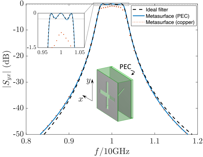
FIG. 6. Polarization-converting reflective metasurface with third-order Chebyshev filter response. The symmetric (across the \hat{x} \pm \hat{y} planes) structure has two metallic sheets and two dielectric layers, on top of a back reflector, with parameters: a = 8.138\text{mm} , w_{1,3}/a = 0.1024 , w_2/a = 6.035 \times 10^{-3} , l_{1,3}/a = 0.7807 , l_2/a = 0.6783 , t_1/a = 0.5142 , t_2/a = 0.0556 , \epsilon_1 = 7.492 , \epsilon_2 = 7.789 .
