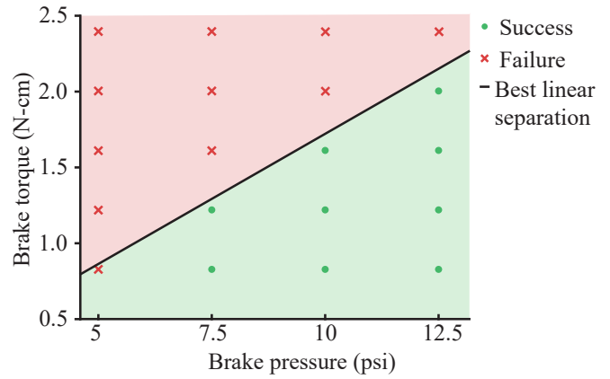
Fig. 7. Brake torque as a function of supplied pressure. Successful and failed trials are shown in green and red, respectively. We also show the best linear approximation to the separation boundary in black.
