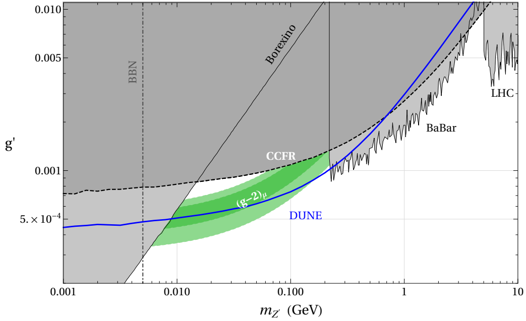
Figure 2.17. Existing constraints and projected DUNE sensitivity in the Z' parameter spaced associated with gauging L_\mu - L_\tau . Shown in green is the region where the (g - 2)_\mu anomaly can be explained at the 2\sigma level. The parameter regions already excluded by existing constraints are shaded in gray and correspond to a CMS search for pp \rightarrow \mu^+\mu^-Z' \rightarrow \mu^+\mu^-\mu^+\mu^- [34] (“LHC”), a BaBar search for e^+e^- \rightarrow \mu^+\mu^-Z' \rightarrow \mu^+\mu^-\mu^+\mu^- [35] (“BaBar”), a previous measurement of the trident cross section [36, 37] (“CCFR”), a measurement of the scattering rate of solar neutrinos on electrons [38–40] (“Borexino”), and bounds from Big Bang Nucleosynthesis [41, 42] (“BBN”). The DUNE sensitivity shown by the solid blue line assumes a measurement of the trident cross section with 40% precision.
