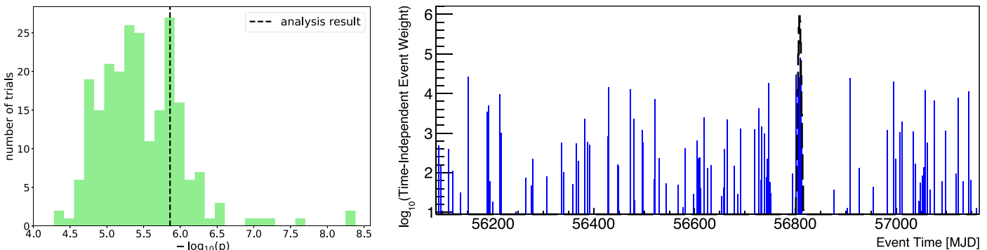
Figure 10. Southern Hemisphere. Left: Expected background p -value distribution obtained from scrambled data in green, compared to the measured most significant pretrial p -value (shown as the black vertical dashed line) in the southern sky. Inferred posttrial p -value is 24.2%. Right: Time-independent event weights, evaluated for the IC86 II-IV data in the Southern Hemisphere, at a source direction x_s defined by the hottest spot (R.A., decl.) = (89°45, -35°95). Best-fit Gaussian time PDF is shown in black (dashed), with mean \hat{T}_0 and sigma \hat{\sigma}_0 .
